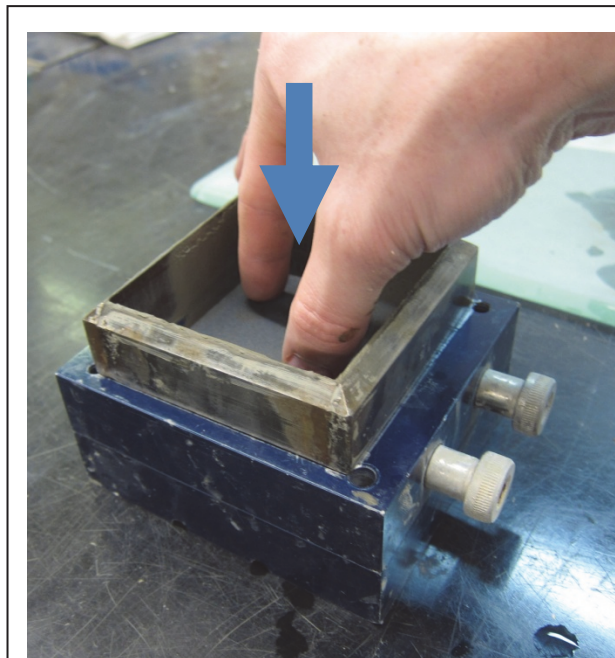
Figure 5. Extruding sample from mold to shear box.
