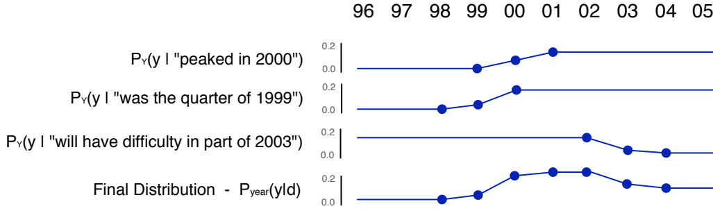
Figure 3: Three year mentions in a document and the distributions output by the learner. The document is from 2002. The dots indicate the before , same , and after relation probabilities. The combination of three constraints results in a final distribution that gives the years 2001 and 2002 the highest probability. This distribution can help a document classifier make a more informed final decision.
