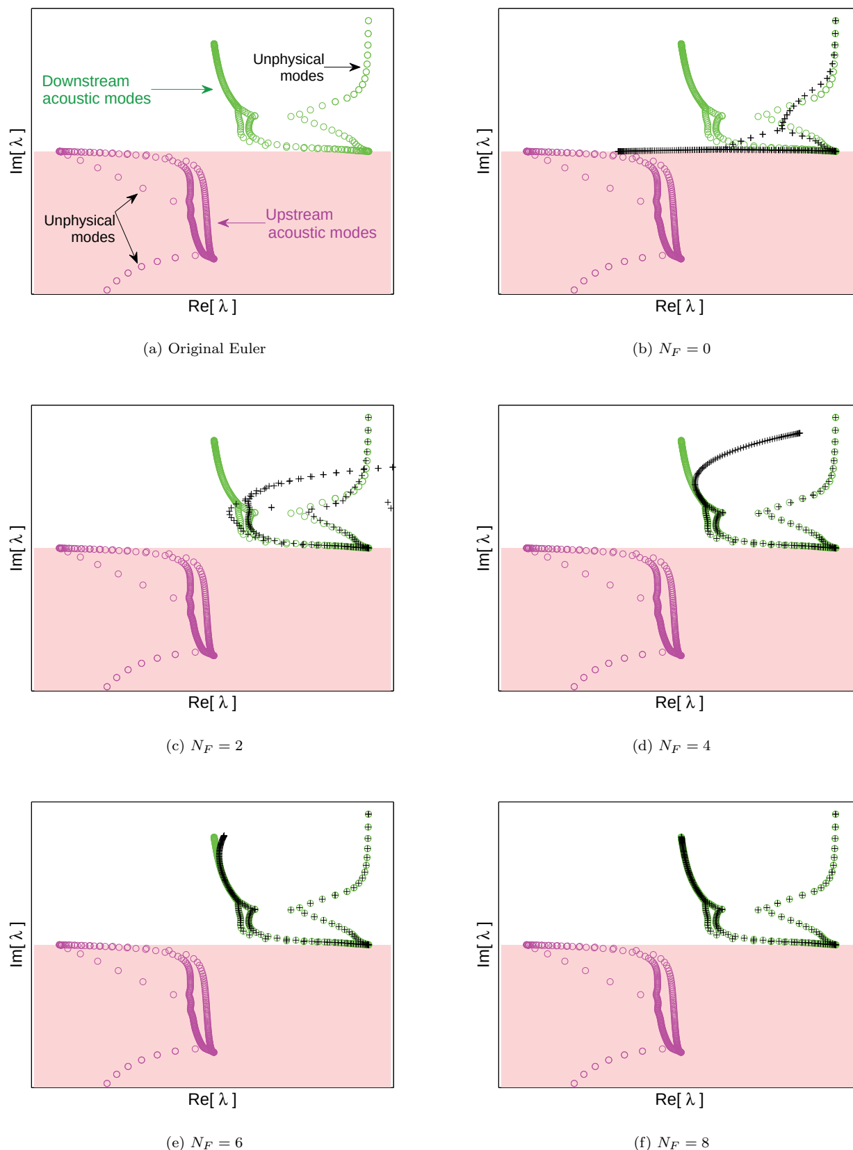
Figure 3: Convergence of the spectrum of the one-way operator to the downstream modes of the original Euler operator. The upstream waves are completely removed and the downstream waves converge rapidly. The circles are the original Euler acoustic modes, and the pluses are the one-way Euler acoustic modes.
