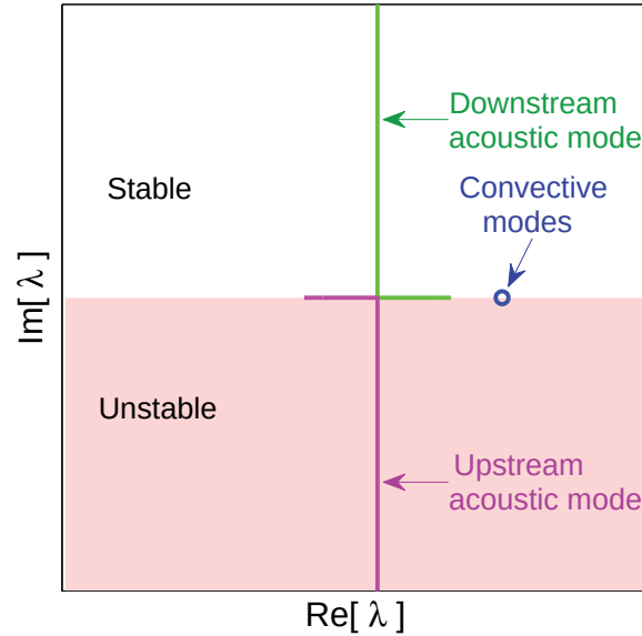
Figure 1: Uniform flow Euler spectrum.
