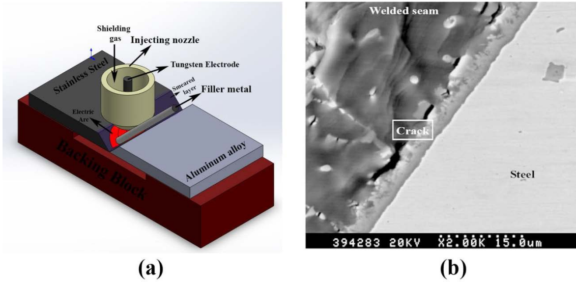
Fig.3. (a) Schematic of the butt TIG welding for joining the aluminum to steel and (b) formation of the cracks at the interface [27, 28].
