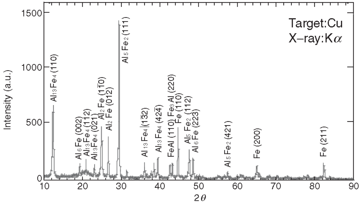
Fig.8. X-ray diffraction pattern shows the presence of different kinds of intermetallics on the fracture surface of the coupons [42].
