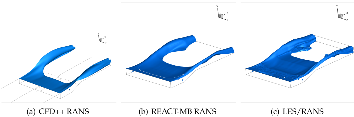
Figure 62: 3D Iso-Surface of 1% Water Mass Fraction
