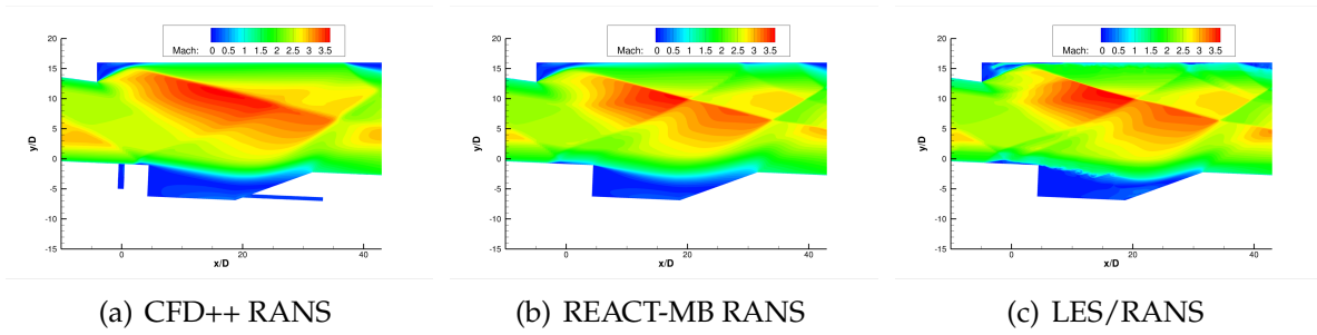
Figure 61: Contours of Mach Number at Center Plane for Shock-On-Jet Case with Cavity Fueling
