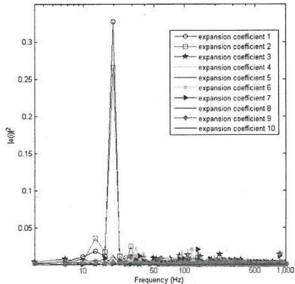
Figure 10: Power spectrum of expansion coefficients of the first 10 modes from the POD analysis. There is a dominant frequency in modes 1 and 2 at ~20 Hz. There are several different peaks in the range of 100-200 Hz for various modes. Modes 3, 7 and 9 (solid symbols) all have a peak at 880 Hz.
