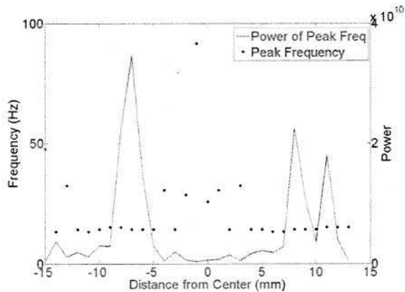
Figure 18: The spectral energy at the peak frequency and that peak frequency varies with location. The shown measurements were made 5 mm downstream of the injector exit. Not shown is the variation in relative dominance of the peaks.
