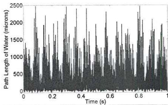
Figure 7: The path length of water in the x-ray beam as a function of time over a 1 second period.
