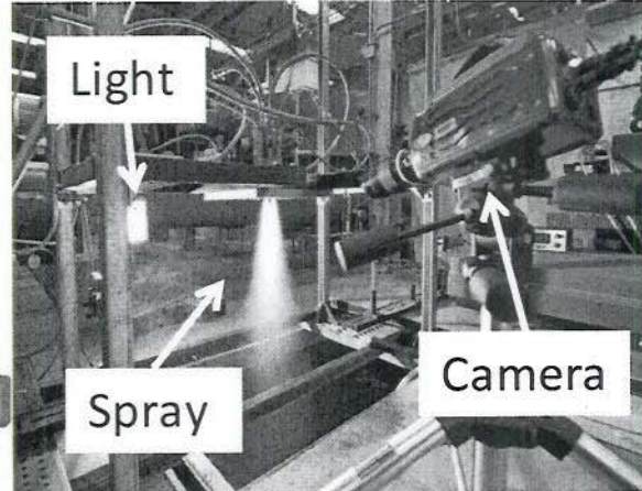
Figure 3: The laser-lighting for the film is shown as a simple cartoon (a). A photograph of the backlighting set-up for the spray imaging is also given (b).
