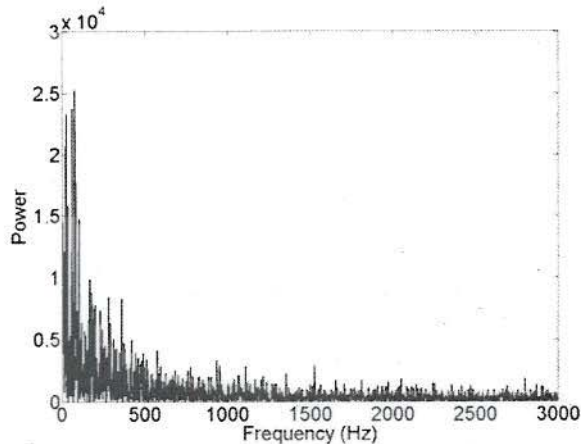
Figure 8: Spectral energy plot from traditional image processing of the film length for a typical case with no dominant frequency.
