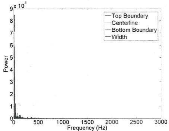
Figure 13: The spectral energy plot for the spray in Case A shows a dominant frequency at 18.02 Hz in all examined parameters except the width. These results are at 5 mm from the injectors exist using image segmentation.
