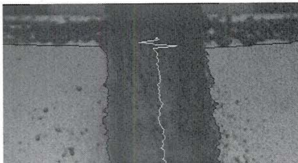
Figure 4: A typical image from the shadowgraphy with the spray boundaries and centerline, as determined by image segregation, shown.
