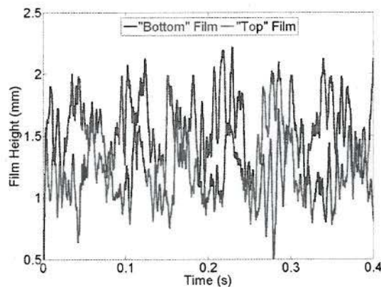
Figure 11: The film height as a function of time (at 9.4 mm) clearly shows a phase lag between the sides of the film.
