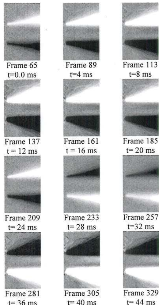
Figure 15: Time series reconstructions of mode 1 of the near-field spray. The POD was performed after subtracting the mean intensity. This mode captures low frequency in the spray which is consistent with the low frequency behavior in the injector as shown in Fig. 12.
