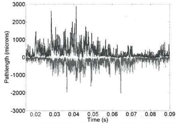
Figure 19: The time-resolved path length of water in the x-ray beam over a single period for locations 5 mm (blue) and 9 mm (red) to the left and right of the centerline. The red data are the negative of the path length to better highlight differences. Data is from 10 mm downstream of the injector outlet.
