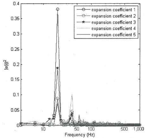
Figure 16: The POD analysis of the spray shows a clear dominant frequency at 20 Hz in modes 1-3, but no evidence of the 880 Hz signal in the first 5 modes.
