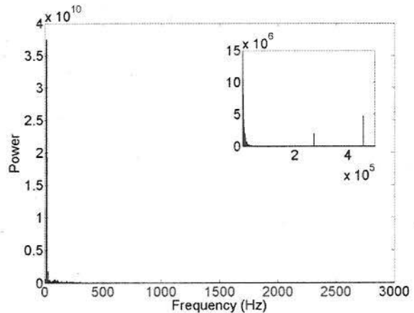
Figure 17: A dominant frequency in the range of 14.3 Hz exists in the x-ray radiography data. There are also several peaks at very high frequency as a result of the x-ray generation process shown in the inset.
