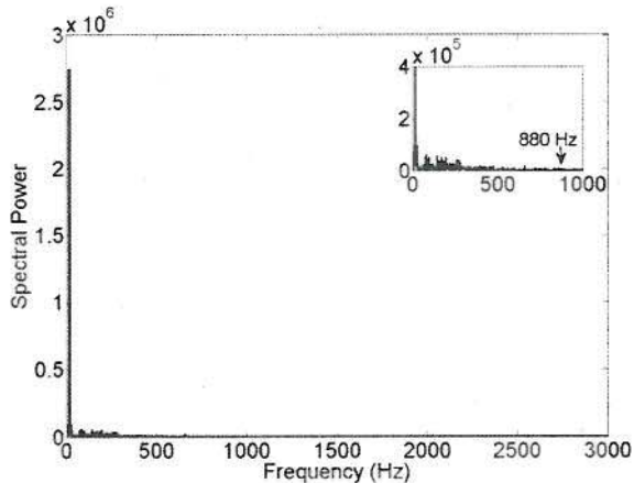
Figure 9: Spectral energy from traditional image processing of the film in Case A shows a dominant frequency in film length variation at 17 Hz. Unlike the POD results (Fig. 10) there is no signature at 880 Hz.
