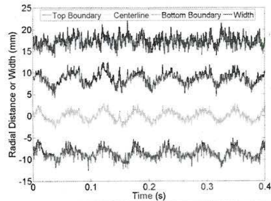
Figure 14: The temporal behavior of Case A indicates a strong periodicity in the edges of centerline of the spray but no organized motion in the width. The behavior 5 mm from the injector exit is shown here.
