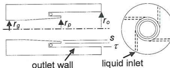
Figure 2: A schematic of a GCSC injector. Table 1 and 2 give the dimensions examined here. r_p is fixed at 6.35 mm.
