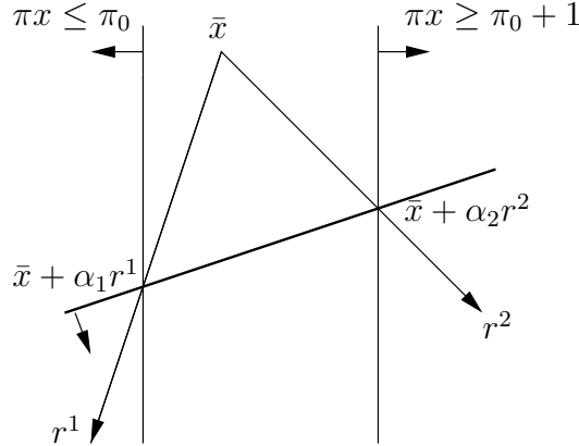
Figure 3: Intersection cut defined by a split
