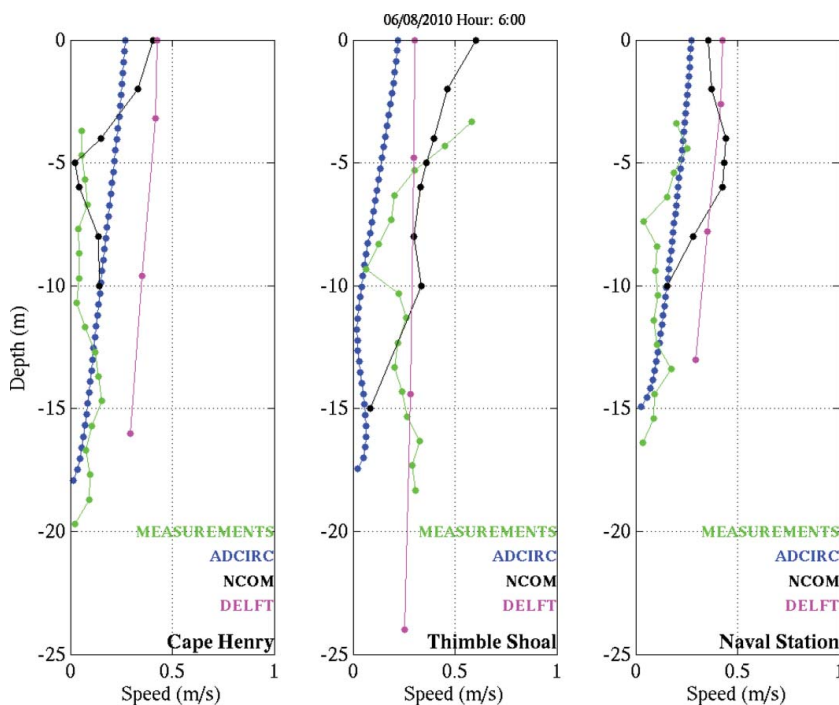
Figure 26. The depth-varying current measurements and model results at Cape Henry, Thimble Shoal and Naval Station NOAA/NOS instrument locations at 0600 hr on June 8, 2010. (Color figure available online.)
