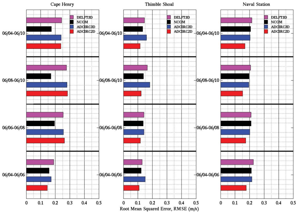
Figure 21. The Root Mean Squared Error (RMSE) of numerical models for depth-integrated currents predictions between June 4 and 10, 2010, at Cape Henry, Thimble Shoal, and Naval Station locations. (Color figure available online.)
