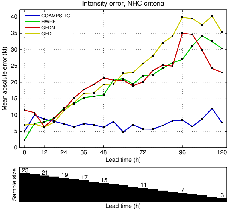
Fig. 4. Wind speed MAE (knots) as a function of forecast time for Hurricane Irene for a homogeneous statistical sample. The numerical models included in this analysis are the Navy’s COAMPS-TC, operational models run by NOAA (HWRF, GFDL), and the Navy’s current operational limited area model (GFDN). The number of cases is shown at the bottom. Only forecasts after Irene has moved away from Hispaniola are shown here. The intensity errors are computed relative to the best track.
