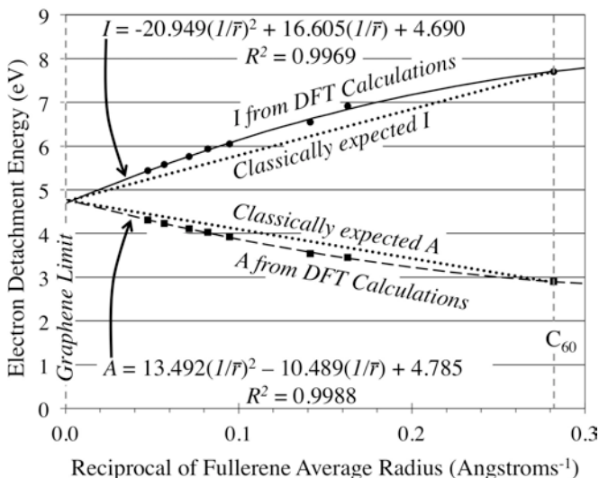
FIG. 2. Icosahedral fullerene ionization potentials (black circles) and electron affinities (black squares), as calculated in this work using density functional theory, are plotted versus reciprocals of the n -carbon neutral molecules' average radii, 1/\bar{r}_n . Values are from part A of Table I. The solid, curved line for ionization potential function I and dashed, curved line for electron affinity function A are determined via second-order regression, for which equations and parameters appear in the figure. Dotted straight lines present scaling of I and A according to a purely classical electrostatic model. Points representing the carbon atom would lie on the solid and dashed lines for I and A , were the axes extended. See text.
