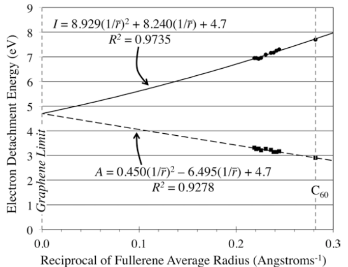
FIG. 3. Nonicosahedral fullerene ionization potentials (black circles) and electron affinities (black squares) are plotted versus reciprocals of the n -carbon neutral molecules' average radii, 1/\bar{r}_n . Values of I_n and A_n are from experimental results reported in the literature and presented in part B of Table I. Values of 1/\bar{r}_n are from theory [14, 15]. As in Fig. 2, the solid, curved line for ionization potential function I and dashed, curved line for electron affinity function A are determined via second-order regression, for which equations and parameters appear in the figure. Unlike the nonlinear regression lines in Fig. 2, above, the lines' intercepts at (1/\bar{r}_n) = 0 were fixed in advance at the value of the graphene work function, 4.7 eV. See text.
