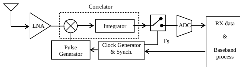
Figure 3: UWB Receiver Block Diagram for a Capsule Endoscope System.
