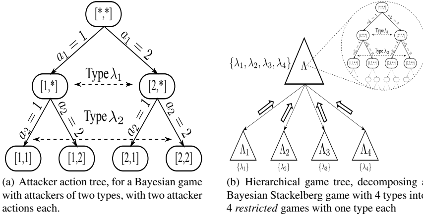
Fig. 6 Hierarchical approach for solving Bayesian Stackelberg games.
