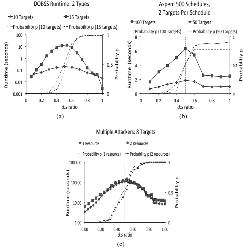
Fig. 8 Average runtime for computing the optimal solution for an example setting for all the three security domains, along with the probability p plotted on the secondary y-axis. The vertical dotted line shows d:s = 0.5 .
