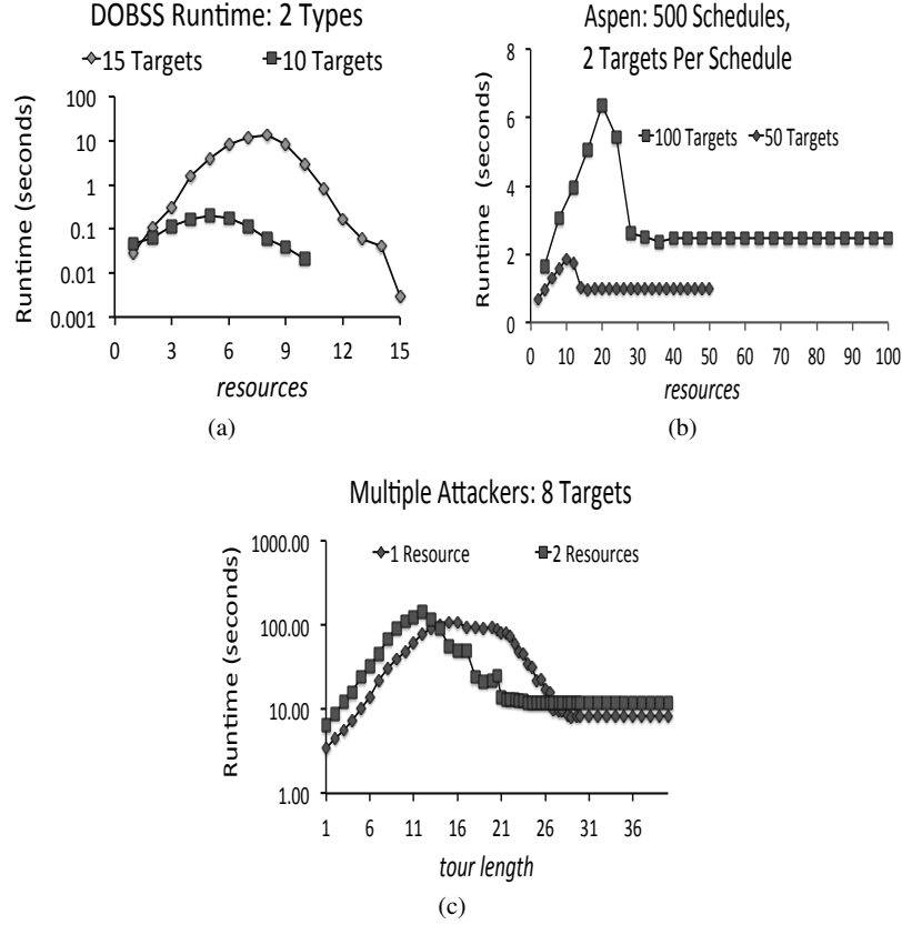
Fig. 7 Average running time of DOBSS, ASPEN and multiple-attacker branch-and-price algorithm for SPNSC, SPARS and SPPC domains respectively.
