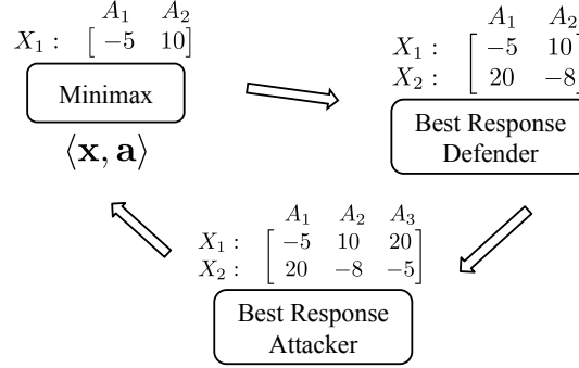
Fig. 5 Strategy Generation employed in RUGGED: The pure strategies for both the defender and the attacker are generated iteratively.
