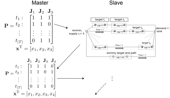
Fig. 4 Strategy generation employed in ASPEN: The schedules for a defender are generated iteratively. The slave problem is a novel minimum-cost integer flow formulation that computes the new pure strategy to be added to \mathbf{P} ; \mathbf{J}_4 is computed and added in this example.
