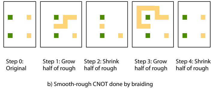
Fig. 31. Smooth-rough CNOT.
