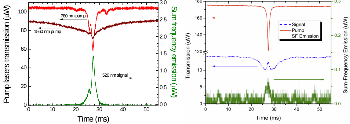
Figure 5. Strongly (left) and weakly (right) pumped SFG in a triply-resonant WGMR. In the weakly-pumped case Zeno-based mode splitting is evident.
