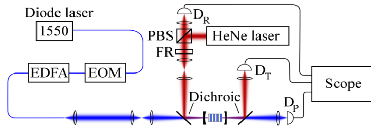
Figure 3. Experimental setup. EDFA: Erbium-Doped Fiber Amplifier. EOM: Electro-Optic Modulator. PBS: Polarizing beam-splitter. FR: Faraday Rotator.
