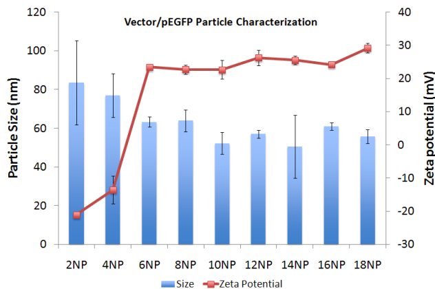
Fig. 2: Various amounts of vector in HEPES buffer were added to 1 \mu g of pDNA (pEGFP) to form complexes at different N:P ratios (N-atoms in vector to P-atoms in pDNA) in a total volume of 100 \mu l deionized water. After 30 minutes of incubation, the size and zeta potential of the complexes were measured and reported as mean \pm s.d., (n=3). Each mean is the average of 15 measurements and n represents the number of separate batches prepared for the measurements.
