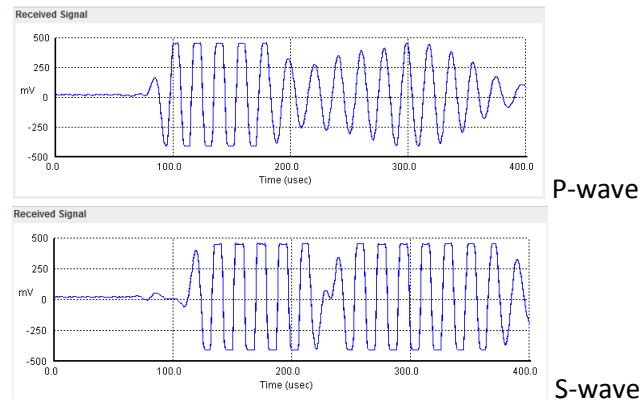
Figure 3: Typical P-wave and S-wave Received Signal
