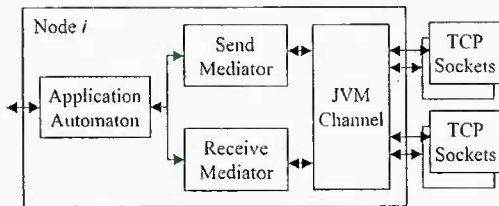
Figure 13: Node automaton.
