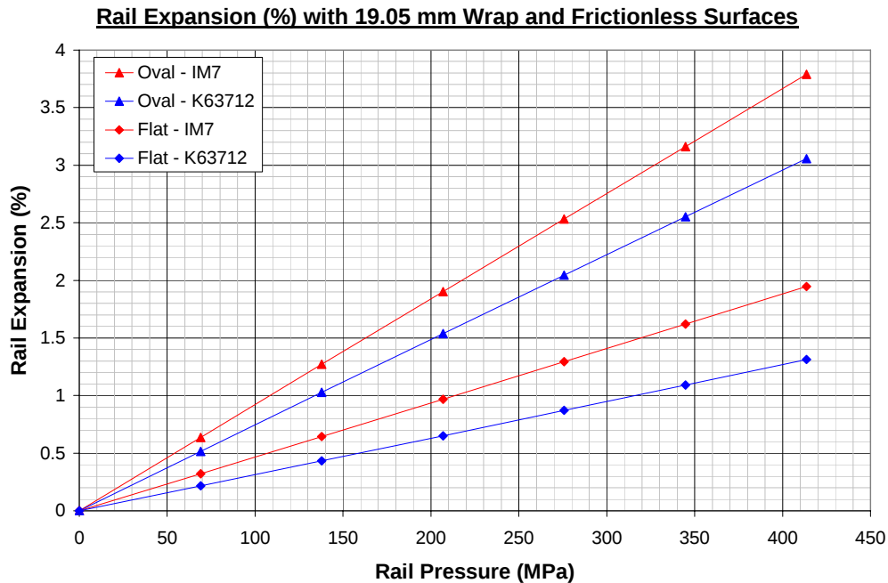
Fig. 8. Wrap material comparison with frictionless surfaces
