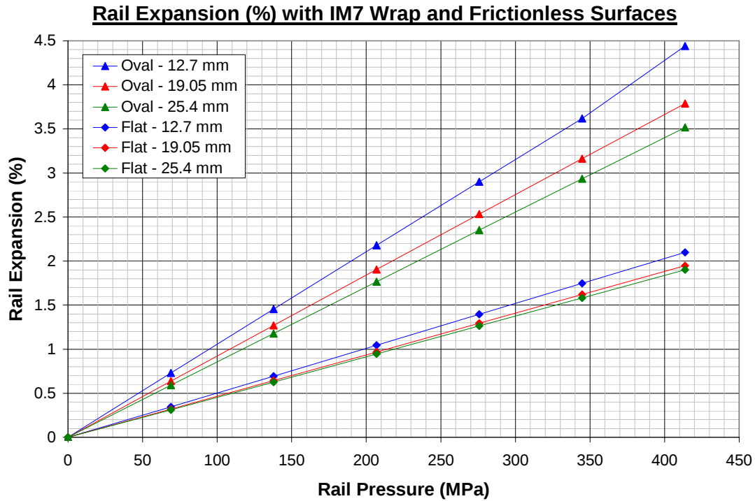
Fig. 6. Results with frictionless contacts
