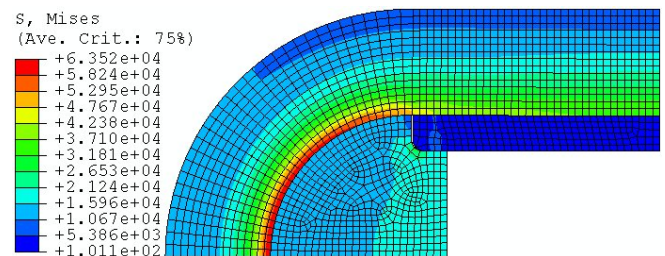
Fig. 5. Von Mises contour plot of flat design with 20 ksi rail pressure (stresses are psi)
