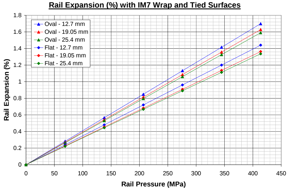
Fig. 7. Results with tied contacts
