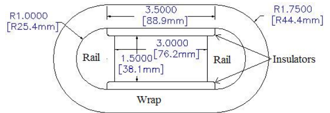
Fig. 2. Flat design
