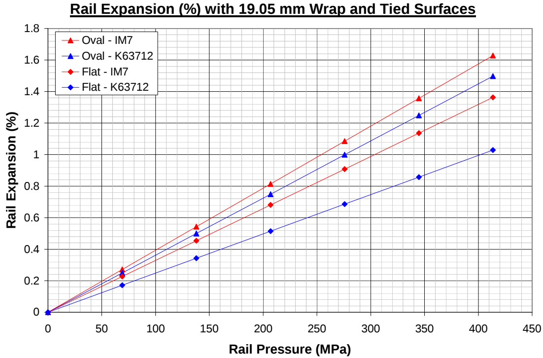
Fig. 9. Wrap material comparison with tied surfaces
