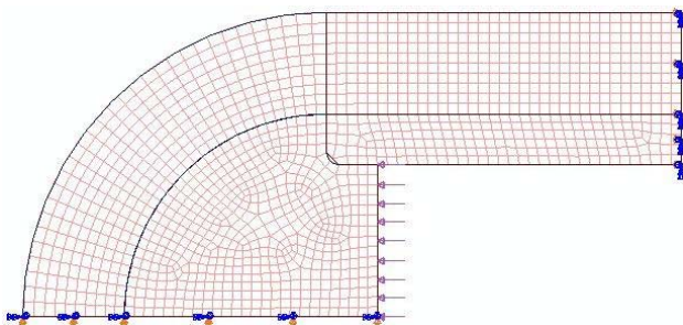
Fig. 3. FEA mesh, loads, and boundary conditions
