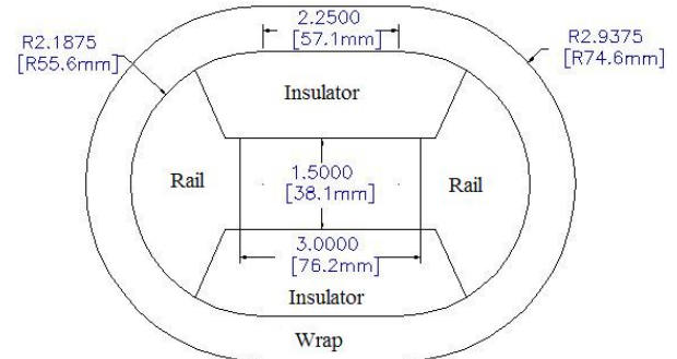
Fig. 1. Oval design
