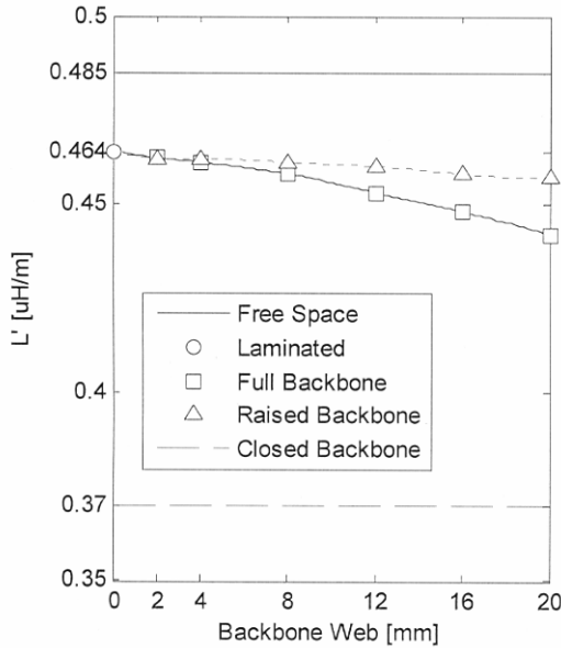
Fig. 2. Computed L' for 50mm Round Backbone Railgun.
