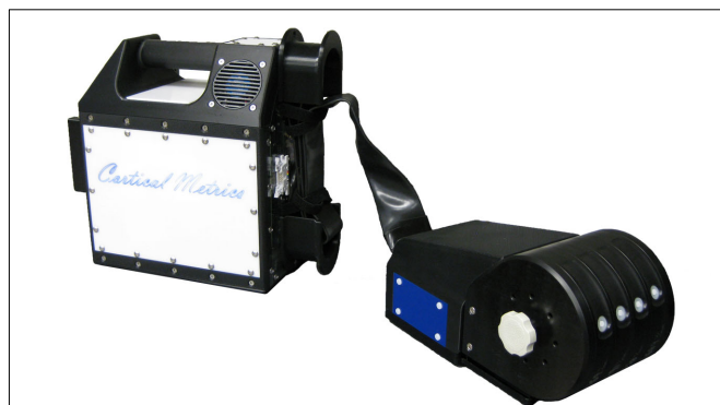
FIGURE 1 | Photo of the multi-site vibrotactile stimulator. During an experimental session, subject was seated comfortably in a chair with right arm resting on the arm rest attached to the head unit of the stimulator. Vibrotactile stimulation was conducted via 5 mm probes that come in touch with subject's index and middle finger.
