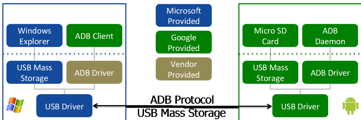
Figure 1 Standard Android USB Communication
