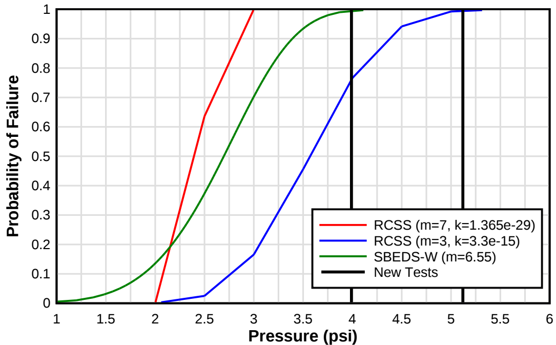
Figure 17. Static Test Validation (60-in × 34-in × 0.115-in Monolithic Hercules® XP)
