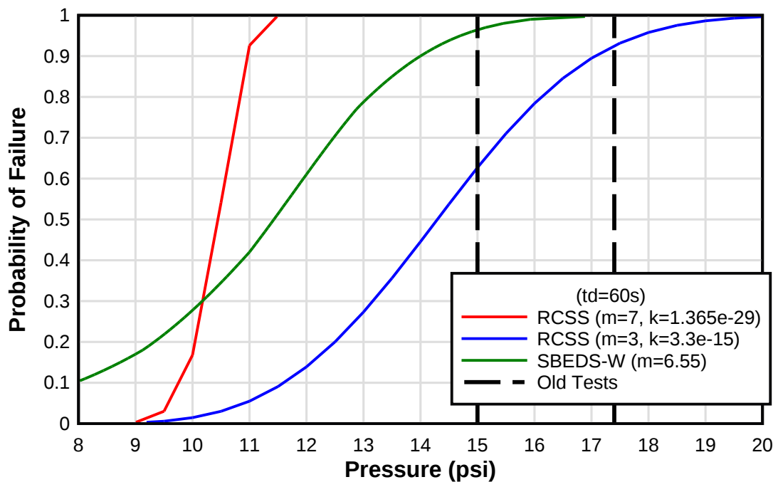
Figure 18. Static Test Validation (39-in × 27-in × 0.190-in Monolithic Hercules® XP)
