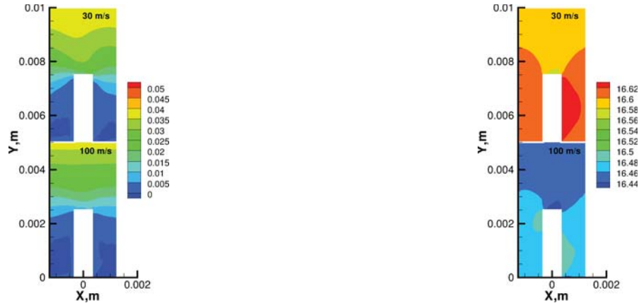
FIGURE 6. Flow velocity normalized by the free stream value (left) and gas pressure (right) for two free stream conditions at an altitude of 60 km.
