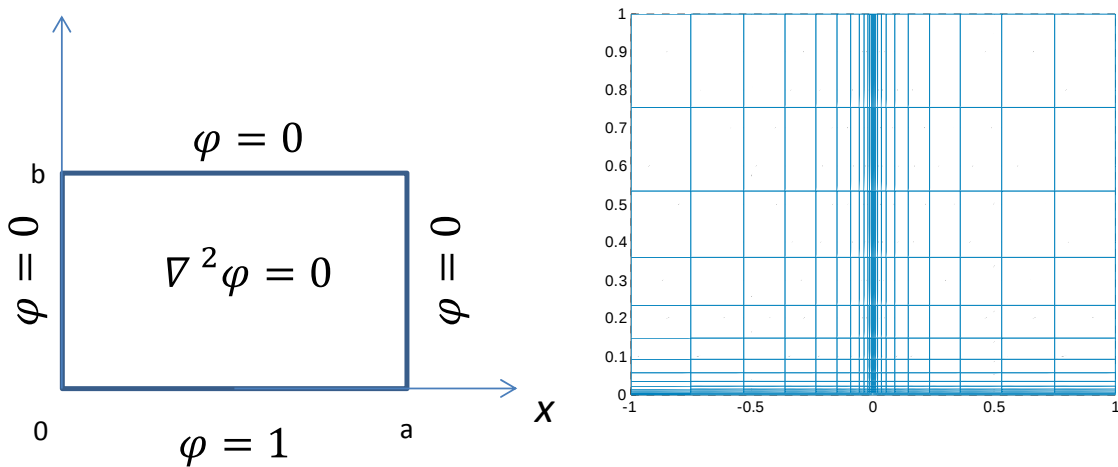
Figure 43. Verification of the force-calculation code: domain and grid. The graphic on the left shows the domain of the test problem, which admits an analytic solution. The numerical grid is shown on the right.
