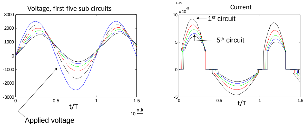
Figure 47. Sample voltage and current computed by the lumped element actuator model. The plot on the left shows the applied voltage and the computed voltage at the first five nodes in the lumped element model actuator solution. The plot on the right shows the corresponding current computed at the first five nodes. The current shows peaks where the plasma ignites.
