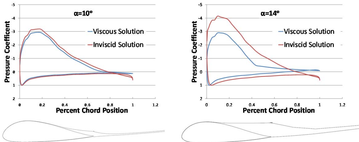
Figure 49. Sample XFOIL calculations. These two graphics show the pressure distribution on the surface of an airfoil at two angles of attack. The airfoil is the seven-tenths radius section of the VP20.
