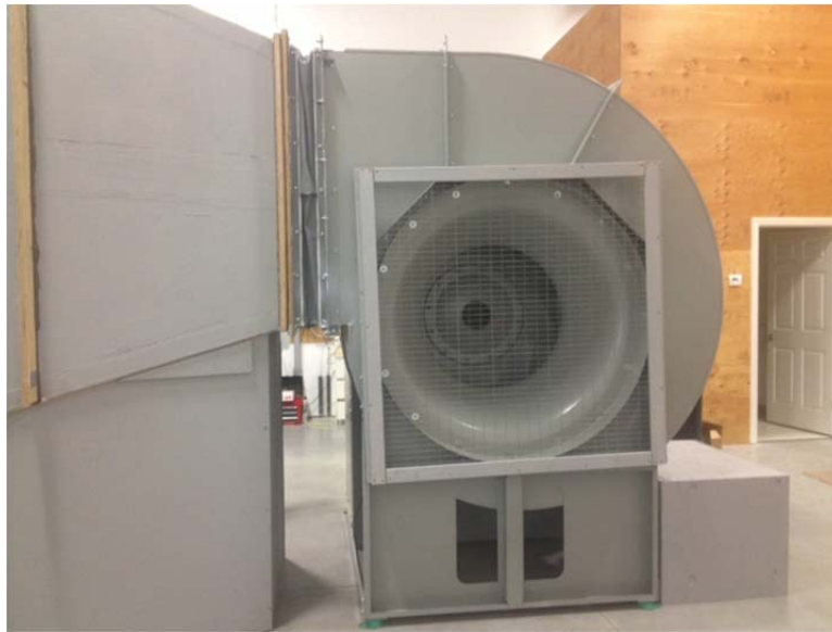
Figure 93. Blower inlet. This picture shows the addition of fencing to prevent ingestion of loose items.
