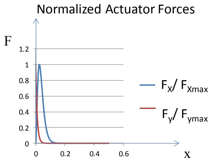
Figure 48. Sample actuator forces computed using the lumped element method. This plot shows forces along the actuator, computed using the lumped element method. These distributed forces can be used as input to FINE™ Marine through the UDF.
