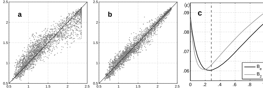
Fig. 8.8 Scatter plots of the true diagonal elements of \mathbf{B}_g (vertical axis) versus their approximations by LH0 (a) and LH1 (b) algorithms. The actual values are multiplied by 10^3 . Near-boundary points are excluded. Right: Diagonal approximation errors as a function of \gamma for the \mathbf{B}_g (black) and \mathbf{B}_2 (gray) models. Dashed line shows the value of \gamma_3^* given by (8.50).
