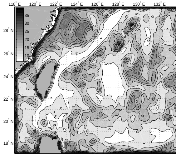
Fig. 8.7 Diagonal elements of \mathbf{B}_g in the Okinawa region at z = 20\text{m} . The actual values are multiplied by 10^4 .
