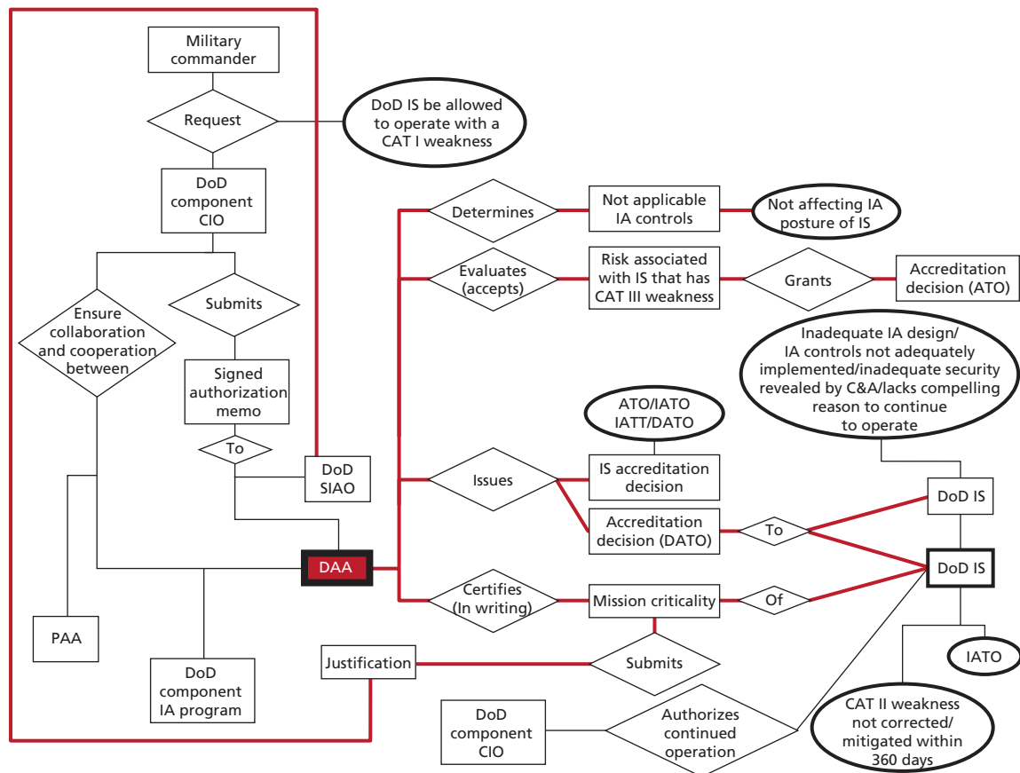
Figure 6.4 ER Diagram for DoDI 8510.01 Focusing on the R&R for the DAA
