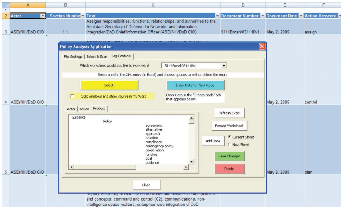
Figure A.7 Tag Controls Interface
