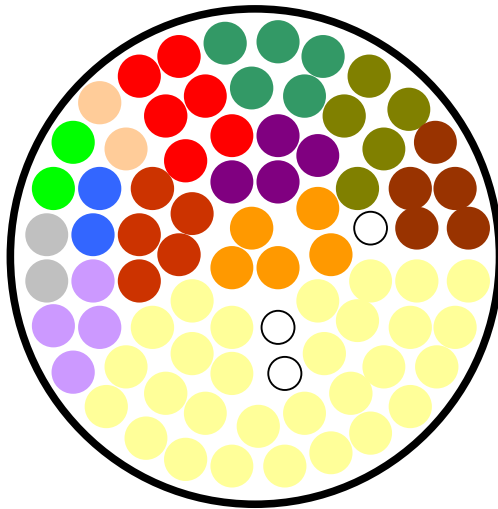
79 pin (20 Devices)
