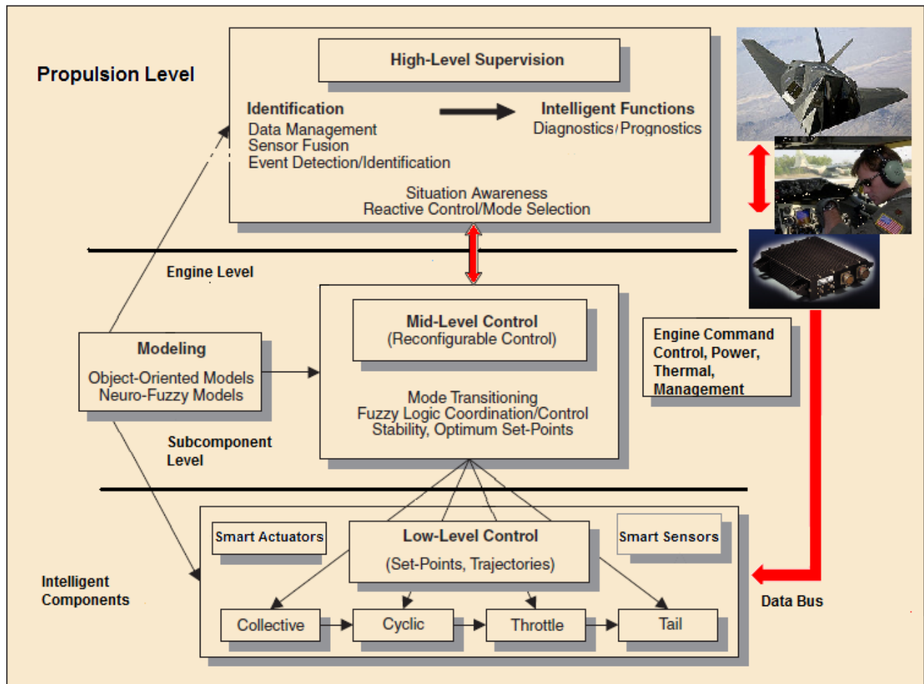
Figure 12: Hierarchical Reconfigurable Distributed Control Architecture
