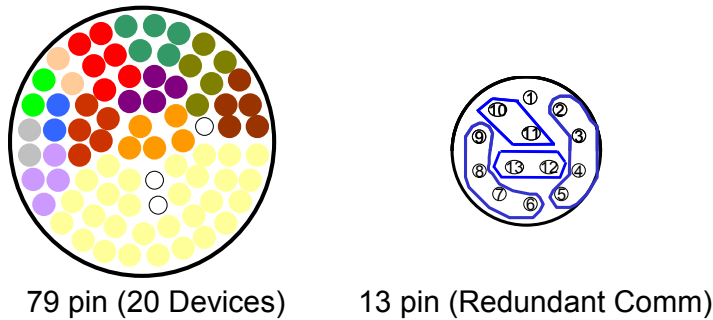
Figure 5: Cable Bundle from Typical FADEC and Replacement
