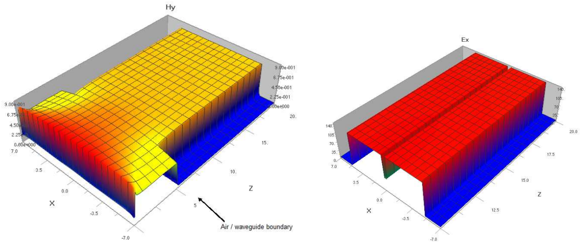
Figure 7. Typical picture of TEM mode at \lambda=300\mu\text{m} , (space dimensions are in microns, amplitude of the fields are shown)
