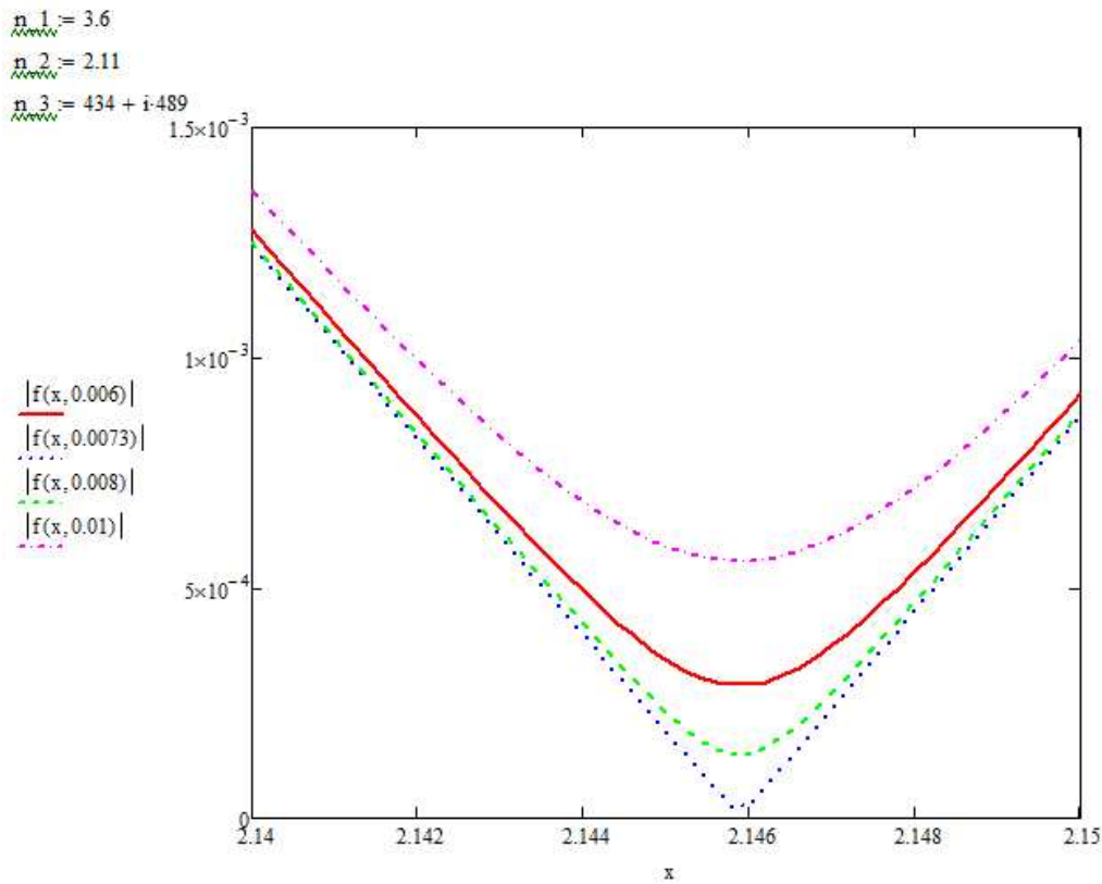
Figure 10. Finding “TEM THz” root graphically \lambda = 214\mu\text{m} . x = \text{Re}(n_{\text{THz}}) .
