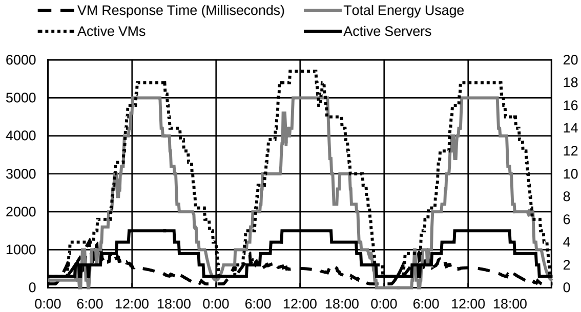
Figure 4: The performance of the Rainbow framework with fifteen minute intervals between communications. The fifteen minute intervals begin to cause an overlap between day-to-day cycles, causing variation in each day's performance.
