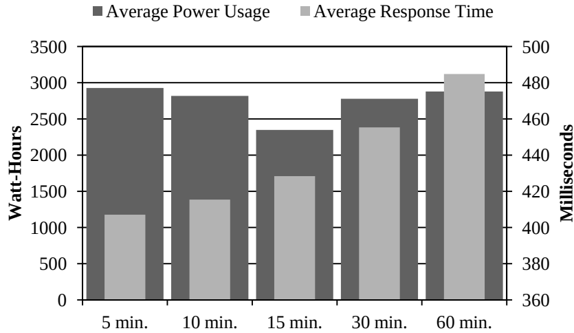
Figure 7: Average power and response time performance of the Rainbow framework across DIL conditions. Under the least degraded environment, the average power usage is 2926 watt-hours and average response time is 407 milliseconds. Increasing the intermittency to ten minutes reduces power usage to 2817 watt-hours, but increases response time to 415 milliseconds. Similarly, the fifteen minute interval decrease power usage and increases response time to 2347 watt-hours and 428 milliseconds respectively. Interestingly, the thirty minute and sixty minute intervals increase both power usage and response time, up to 2877 watt-hours and 484 milliseconds.
