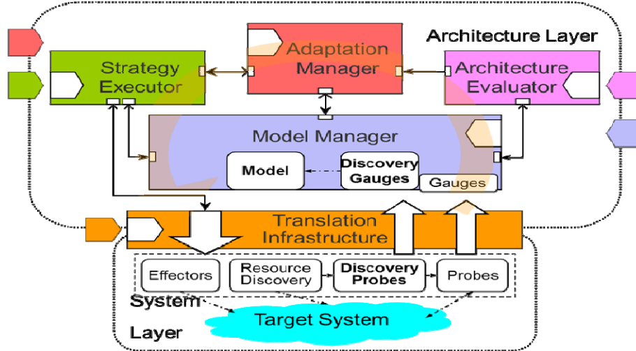
Image 2: Two components were added to the Rainbow framework to facilitate discovery. The first item is Discovery Gauges that directly interact with the ACME model to generate necessary model components to represent the discovered elements of the target system. The information for the creation of architectural elements comes from Discovery Probes, which are responsible for initializing the Probes that report data about the target system. In this way, whenever any component begins to report data, it first registers through discovery to generate matching architecture in the ACME model.
