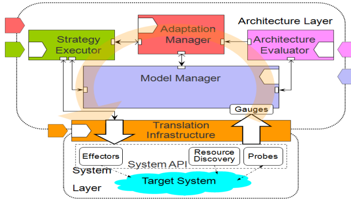
Image 1: The Rainbow Framework (from [18]) consists of four primary components: The Model Manager, the Architecture Evaluator, the Adaptation Manager, and the Strategy Executor. In addition, for each target system being managed, there is a Translation Infrastructure that provides the means to send data to the Rainbow framework and for Rainbow to effect changes in the target system.
