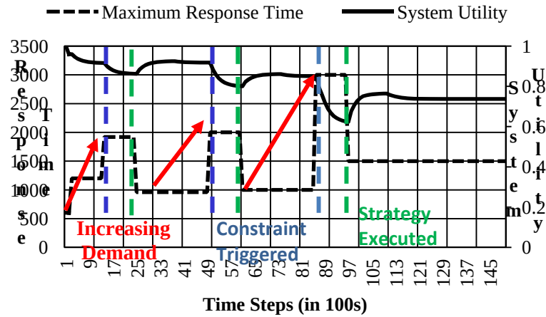
Figure 1: This example demonstrates the effect of Rainbow’s autonomic management on the system. Based upon demand on the system, response time for services begin to increase. Eventually, the measured response time violates the constraints defined in the ACME model managed by rainbow. The Adaptation Manager then activates a particular strategy that addresses the increased demand and the Strategy Executor effects the desired changed in the target system, leading to a decrease in response time.
