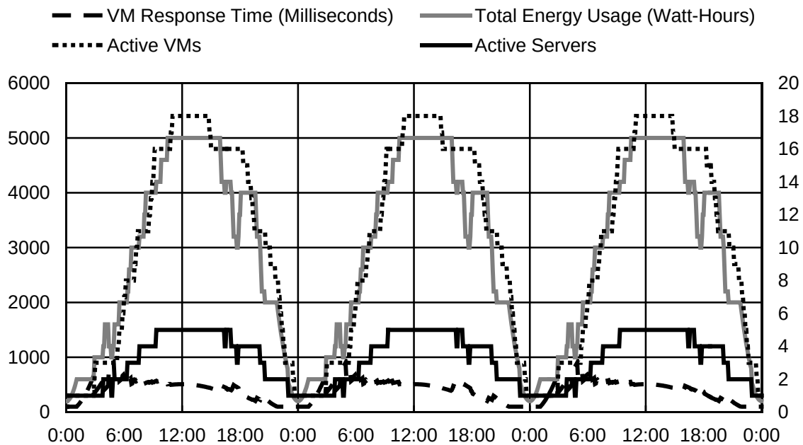
Figure 2: The performance of the Rainbow framework with five minute intervals between communications. In this environment with short intervals between communication, Rainbow can effectively activate and deactivate resources, such as virtual machines (VMs) and servers, as needed and in a timely fashion.
