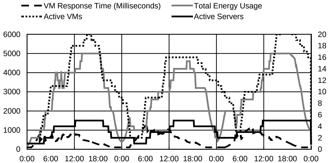
Figure 6: The performance of the Rainbow framework with sixty minute intervals between communications. The most degraded communications causes Rainbow to request resources much later than required and keep them activate longer than necessary. The overlapping interaction causes Rainbow to have too many resources online for periods of low activity.
