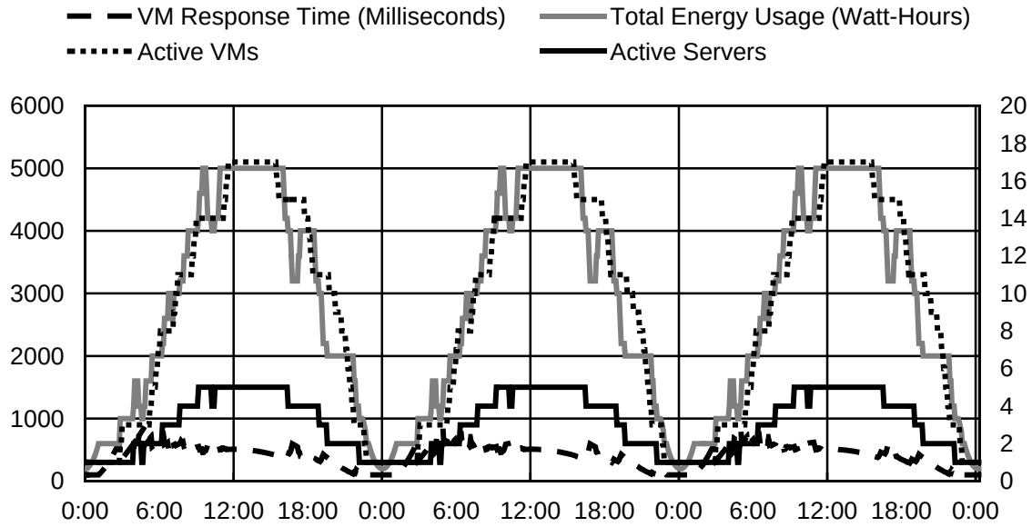
Figure 3: The performance of the Rainbow framework with ten minute intervals between communications. The slightly longer intervals between communication causes Rainbow to lag slightly behind in adding needed resources.
