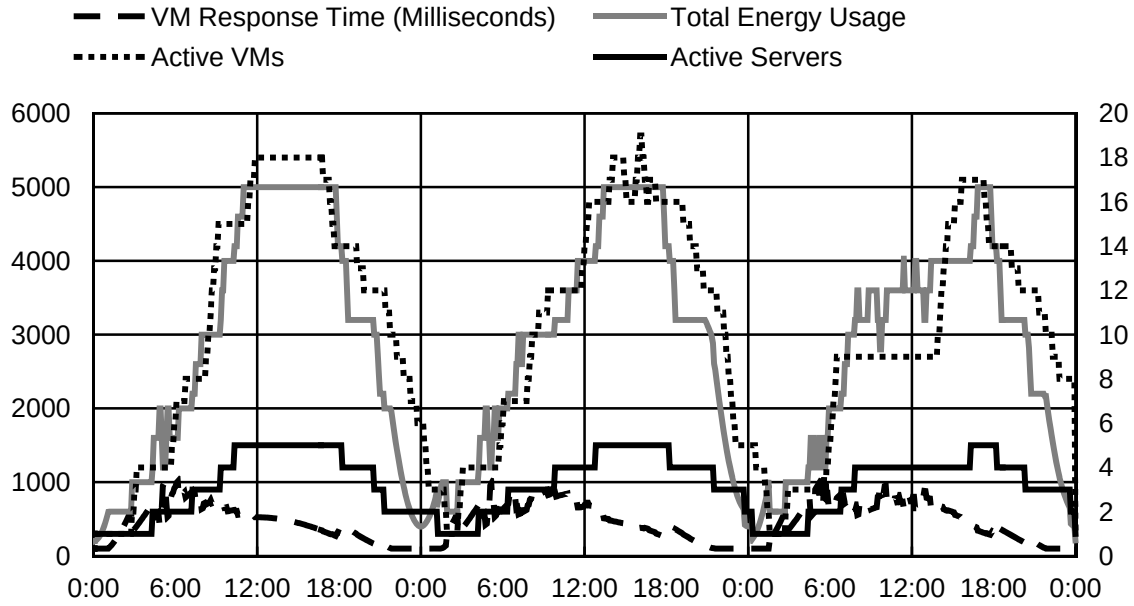
Figure 5: The performance of the Rainbow framework with thirty minute intervals between communications. Increasingly, the DIL environment causes destabilization in Rainbow’s management of the target system.
