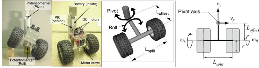
Fig. 3 Assembly of Active Split Offset Caster module (left) and schematic illustration of ASOC (middle and right)
