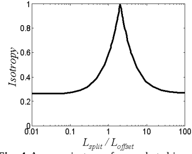
Fig. 4 Average isotropy for a robot driven by ASOC modules as a function of L_{split} / L_{offset} (from [13])
