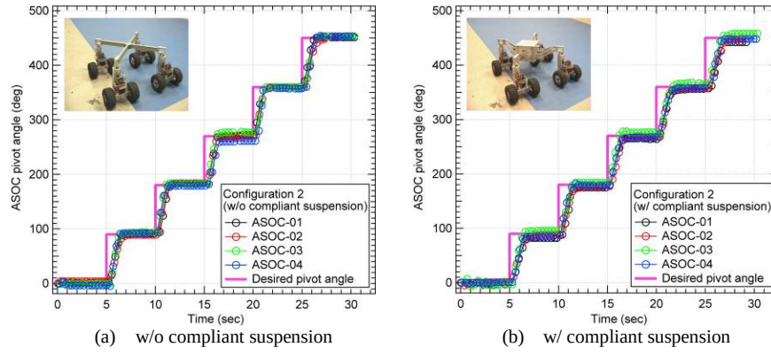
Fig. 12 Time history of the pivot angle for mobility evaluation (Configuration 2).
