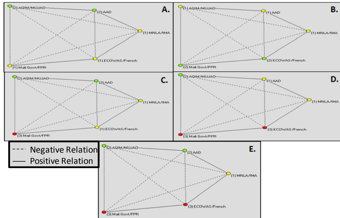
Figure 28: Five different partitions of the reduced network, each having two inconsistencies. Graphs A and B are partitioned into two subsets, Graphs C, D, and E are partitioned into three subsets.
