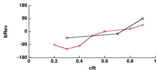
Figure 32. Comparison of NFAC blade torsion ( C_{T0} ) harmonic phases with flight test (c8424, R47P21).
