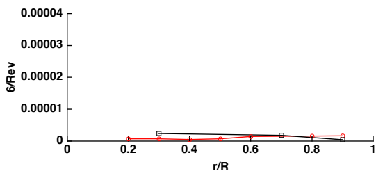
Figure 31. Comparison of NFAC blade torsion ( C_{T0} ) harmonic magnitudes with flight test (c8424, R47P21).
