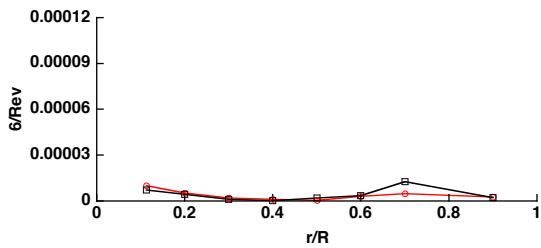
Figure 29. Comparison of NFAC blade flap bending ( C_{FB} ) harmonic magnitudes with flight test (c8424, R47P21).
