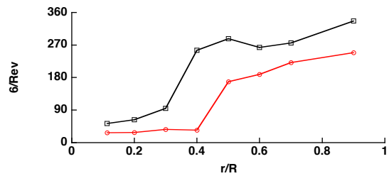
Figure 30. Comparison of NFAC blade flap bending ( C_{FB} ) harmonic phases with flight test (c8424, R47P21).
