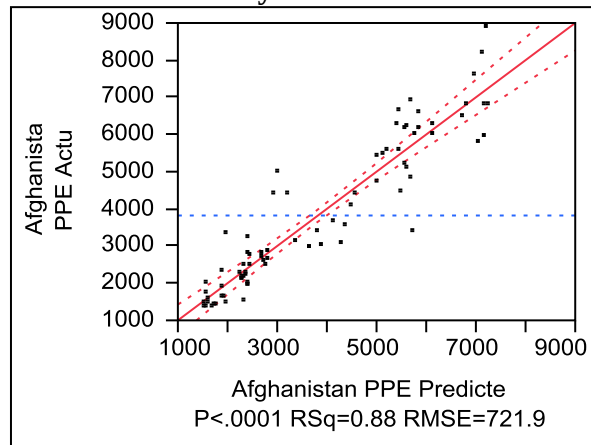
Response Afghanistan PPE Whole Model Actual by Predicted Plot
