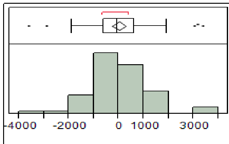
Figure 11: Histogram of Residuals (Iraq GDSS2)
