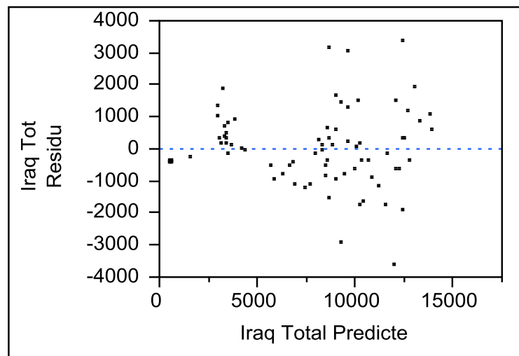
Figure 9: Residual by Predicted Plot (Iraq GDSS2)
