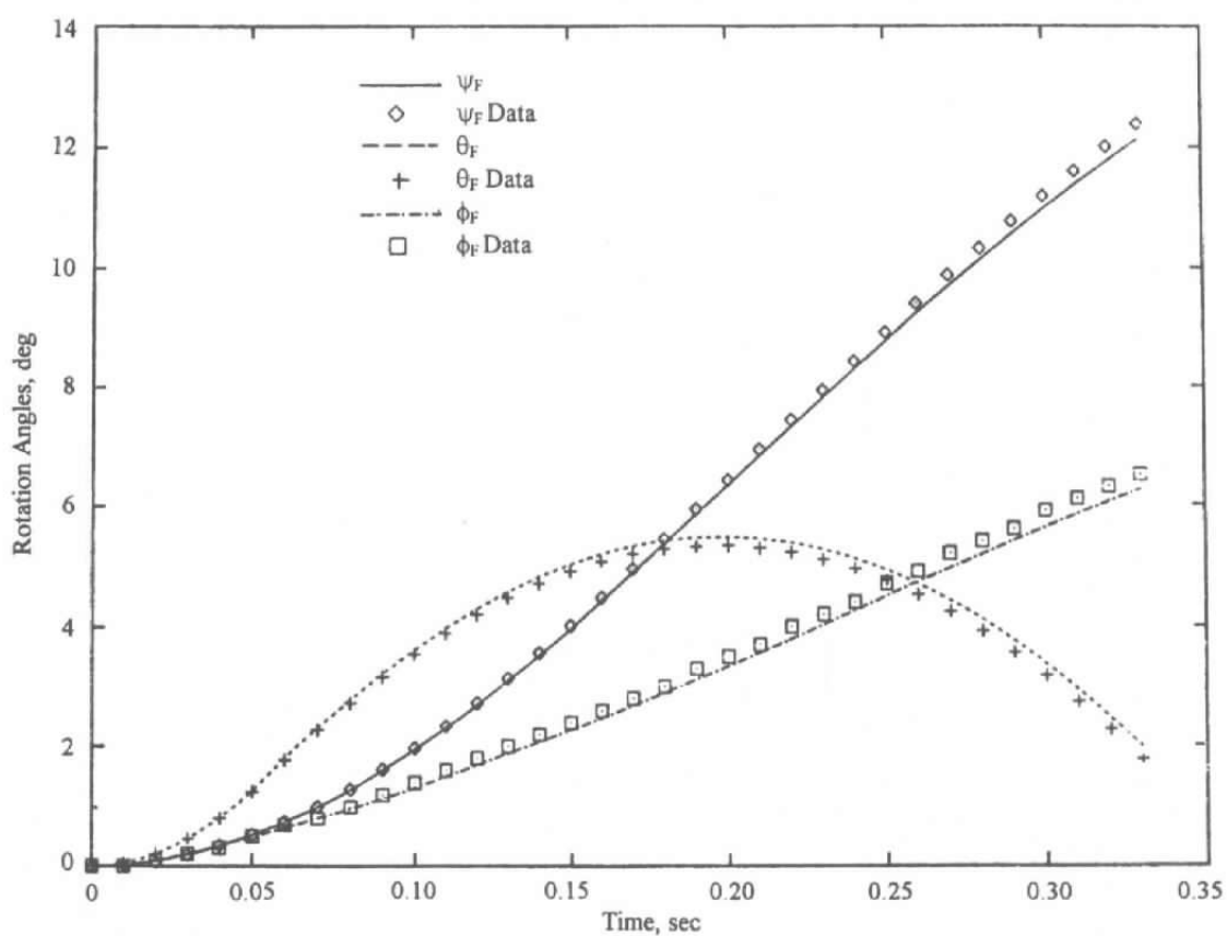
c. Rotational angles with respect to flight axis system
