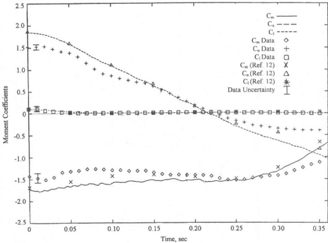
a. Moment coefficients in body axis system
