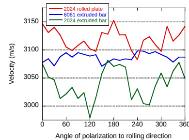
Figure 32. Series of aluminum alloys from laser line source-in/laser-out method. Al2024 exhibits measureable anisotropy, while 6061 appears to maintain isotropic behavior.
