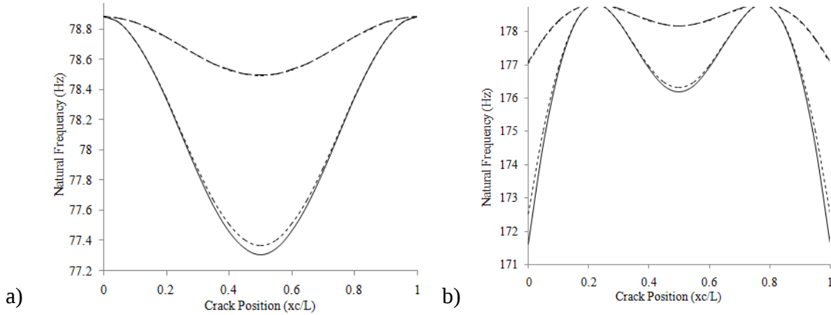
Figure 26. Resonant frequency of the 1 st mode of the beam vs. crack position along the beam for a) simply supported and b) fixed-fixed boundary conditions.
