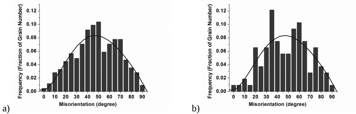
Figure 8. Statistical distribution used for misorientation feature identification a) actual data; b) example of generated SVE.
