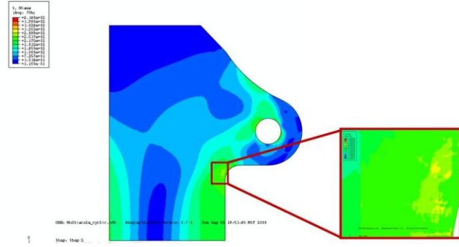
Figure 12. Mises stress distribution of lug joint.
