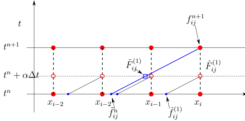
Figure 23: Construction of two-stage stiffly-accurate DIRK. The first stage is computed on the grid points (t^n + \alpha\Delta t, x_i) (empty red circle) by an implicit step. The RK fluxes are computed on the same points, and then interpolated to points (t^n + \alpha\Delta t, x_i - (1 - \alpha)v_j\Delta t) , denoted by a small blue square. Finally, the second stage value along the characteristics is computed on the grid. Such stage value corresponds to the numerical solution implicit scheme
