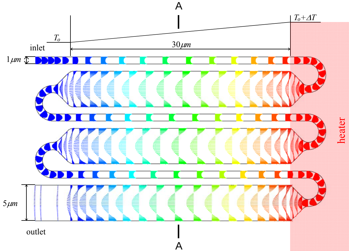
Figure 20: An illustration of a central 3 stage heated Knudsen pump and gas flow velocity vectors in the pump. Red colour indicates hot and blue cold. The temperature on the walls is linearly distributed.
