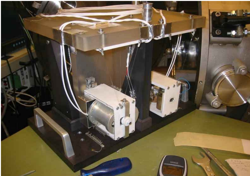
Figure 6: Micro Thrust Balance at EPL.
