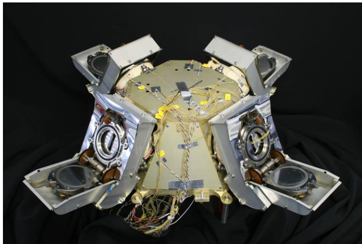
Figure 4: FEEP thrusters for LISA-Pathfinder Concept and Demonstrator
