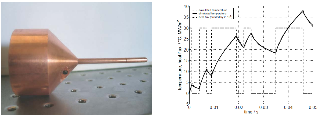
Figure 8: Miniaturized heat flux sensor based on the Non-Integer System Identification (NISI) Method (left) and calibration data of the sensor (right) [71]
