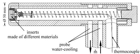
Figure 5: Transient heat flux probe.
