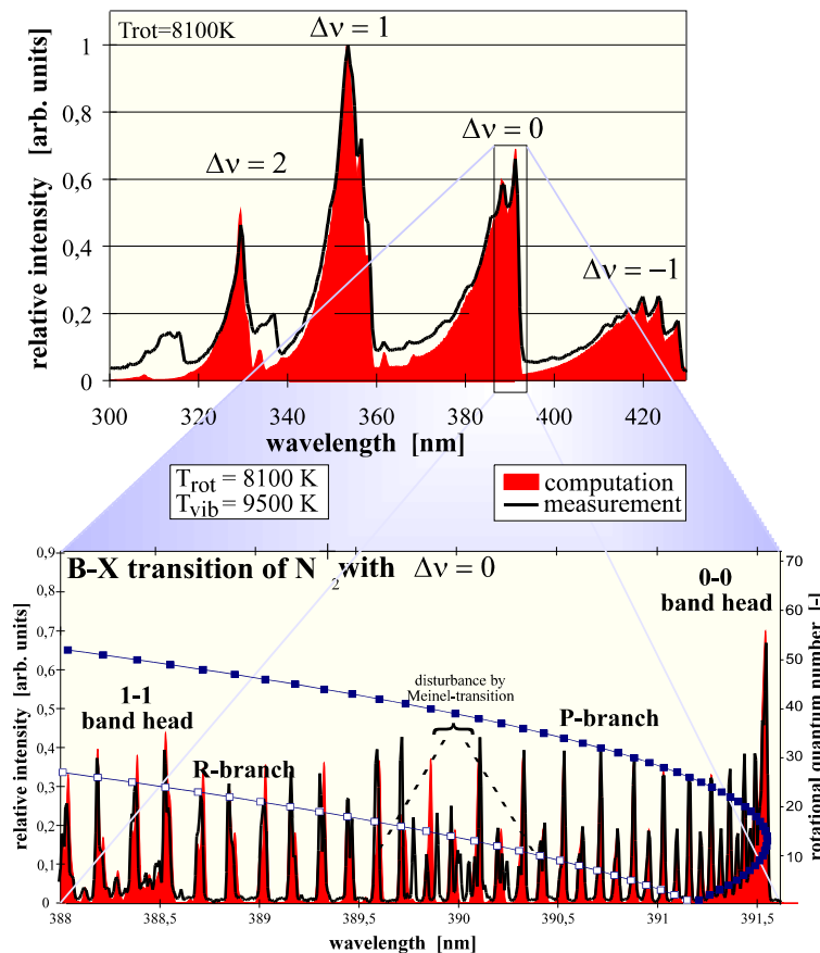
Figure 43: Band structure of the N_2^+ -molecule measured in front of a hot SiC material sample ( T_{Wall} = 1580^\circ C ).
