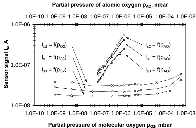
Figure 29: Atomic oxygen sensor signal depending on atomic and molecular oxygen partial pressures.
