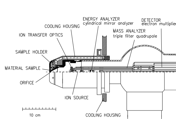
Figure 19: MS configuration for erosion investigation
