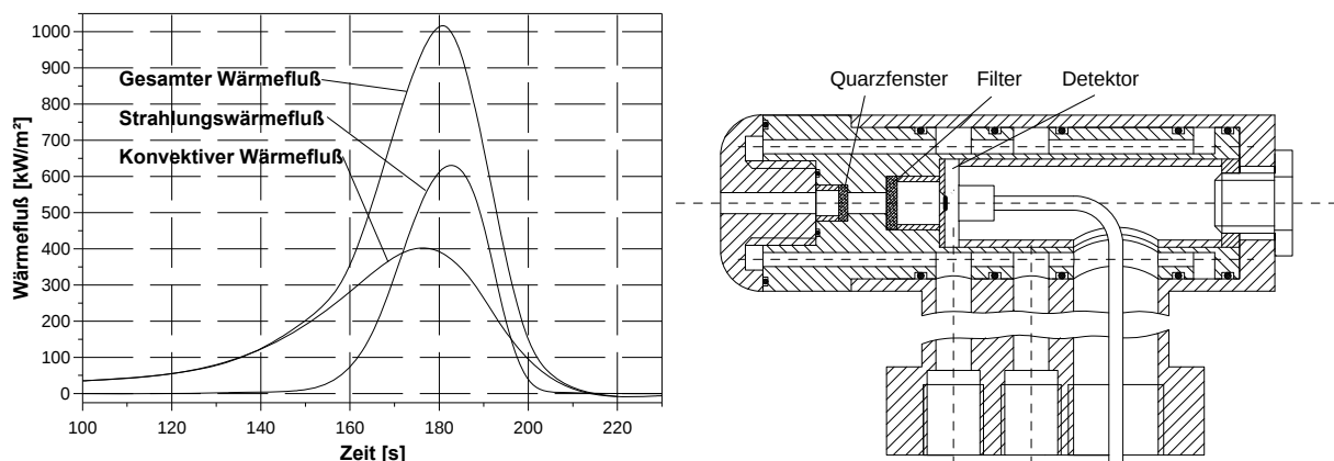
Figure 36: Left: Calculated heat fluxes for the entry of the Huygens probe into the \text{N}_2/\text{Ar}/\text{CH}_4 atmosphere of the Saturn moon Titan (without catalytic effects). Right: Radiometer probe with dismountable quartz window and filter
