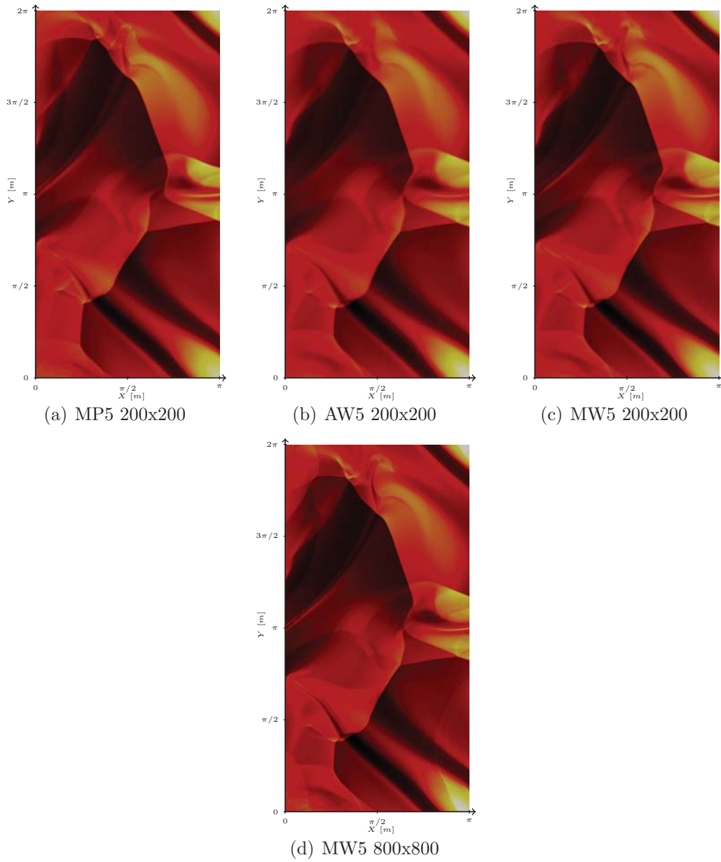
Figure 4.16: Density distribution for Orszag-Tang problem for x \times y \in [0, \pi]m \times [0, 2\pi]m CFL = 0.4, runtime = 3 s, \min \max .
