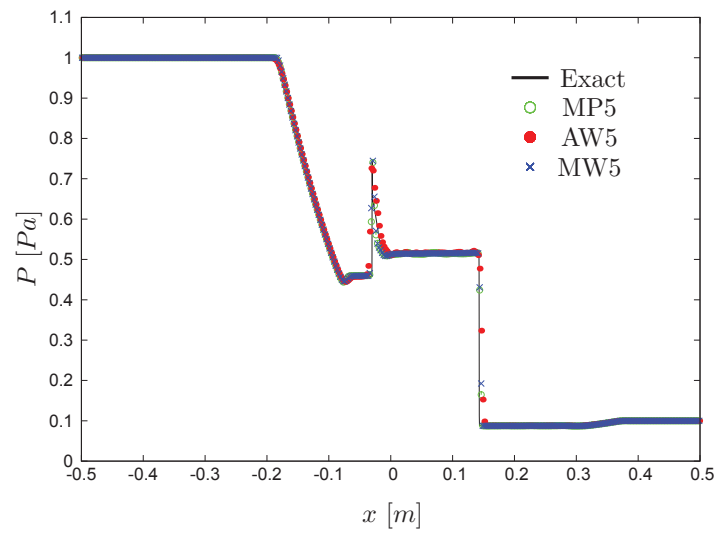
Figure 4.14: Pressure distribution of the Brio-Wu[60] problem using MP5, AW5 and MW5, \Delta x = 2.5 \times 10^{-3}m , CFL = 0.4, runtime = 100ms
