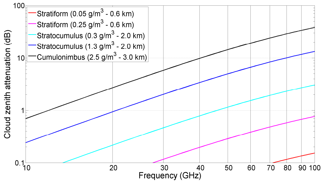
Figure 2-3. Zenith attenuation for different type of clouds as a function of frequency between 10 and 100 GHz (refer to the figure's legend for more details on the values employed in the calculation)
