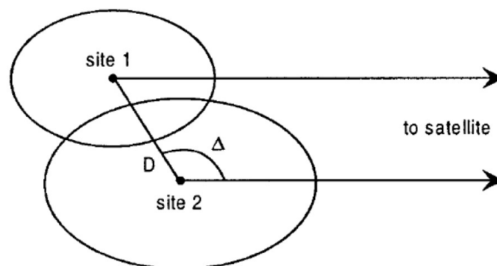
Figure 4-25. Schematic representation of a dual site diversity system ( D and \Delta are respectively the baseline distance and orientation); the kernels of the two links are represented by the ellipses
