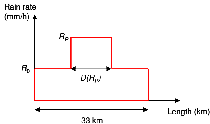
Figure 4-1. Reference model for the rain cell in the Assis-Einloft model
