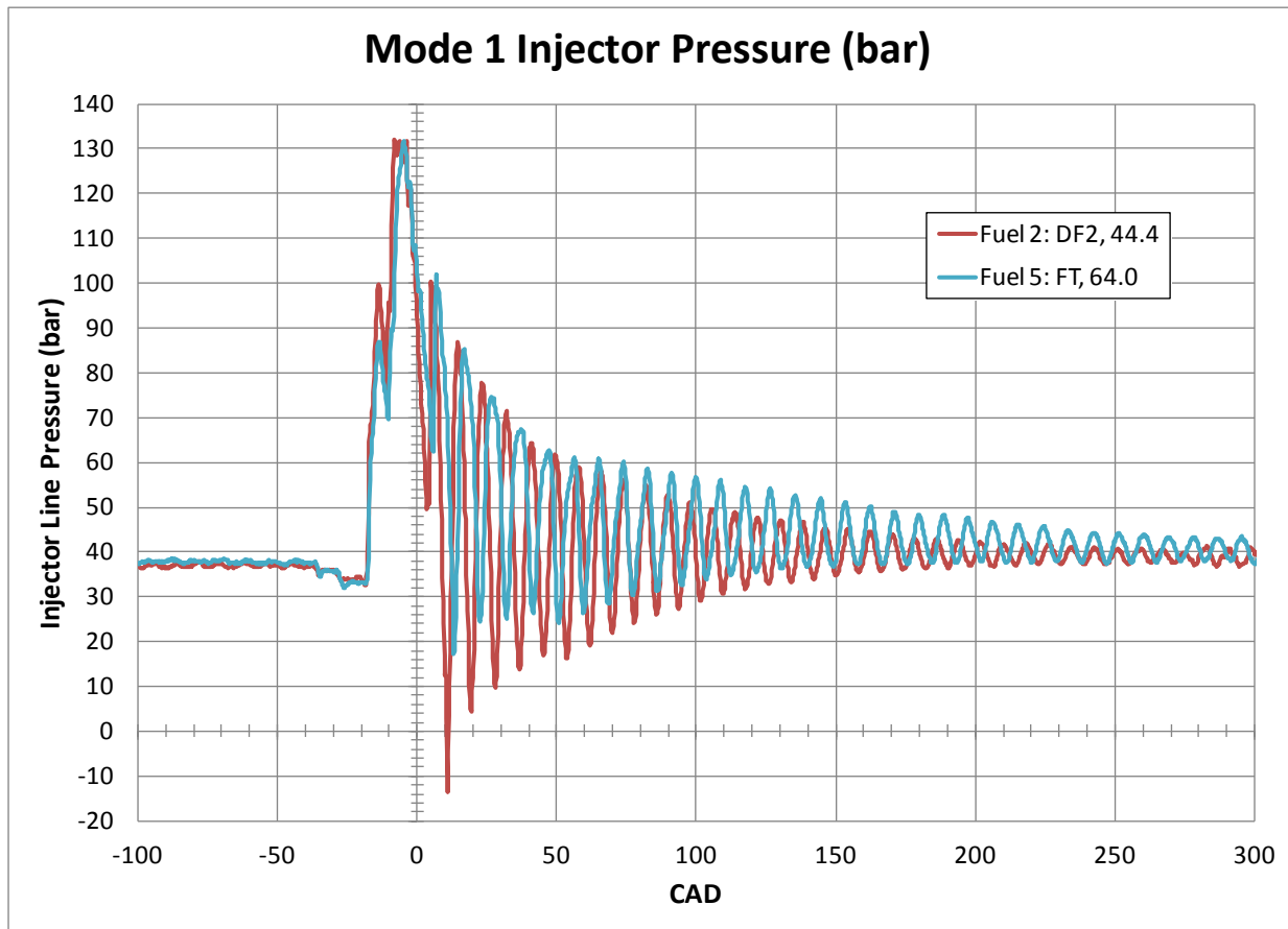
Figure 33. GEP 6.5T ESC Mode 1 Injection Line Ringing Frequency
