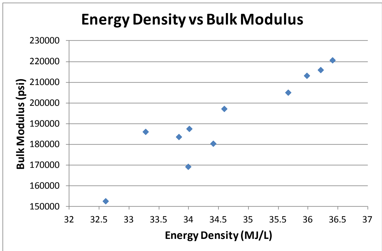
Figure 32. Fuel Bulk Modulus vs. Energy Density
