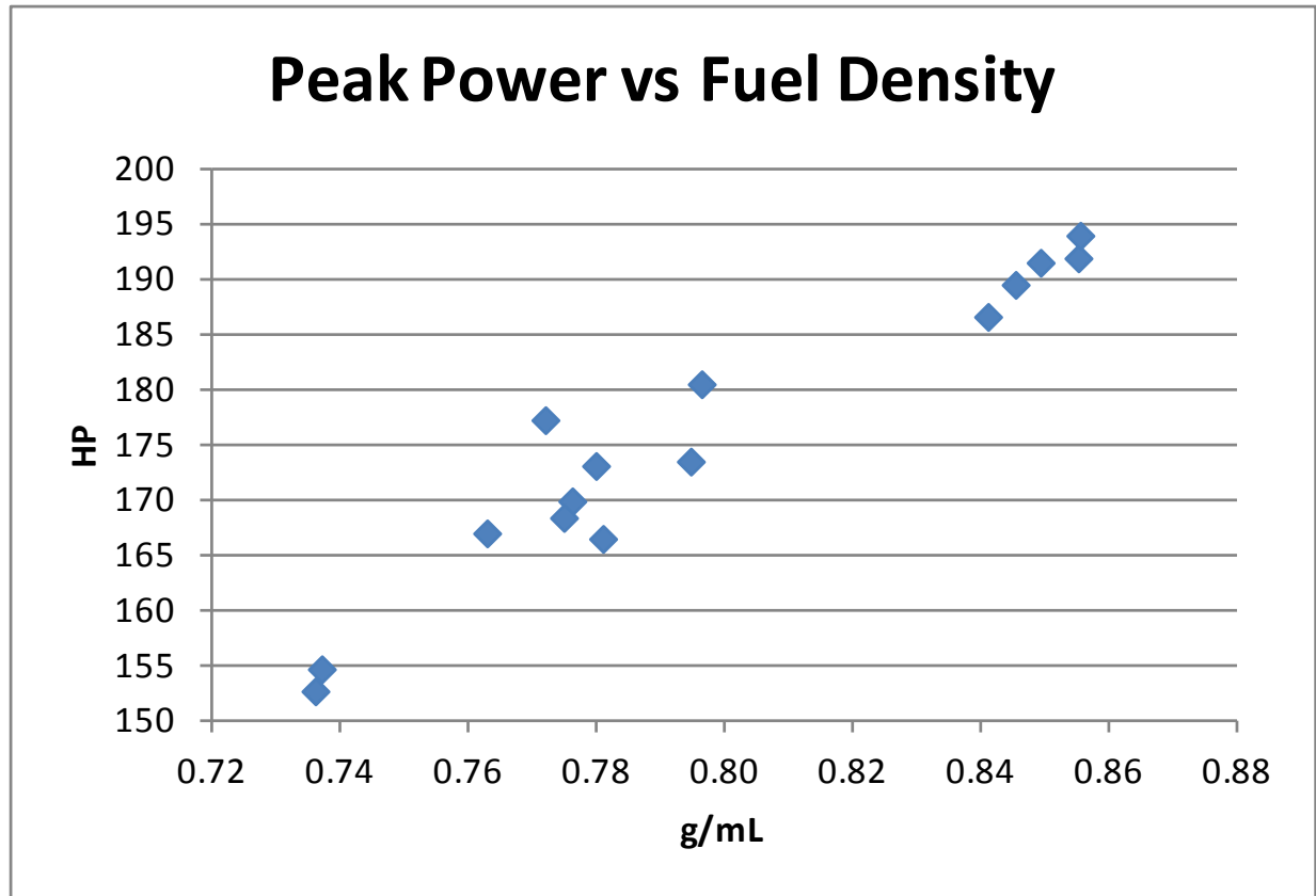
Figure 19. GEP 6.5T Peak Power vs. Fuel Density
