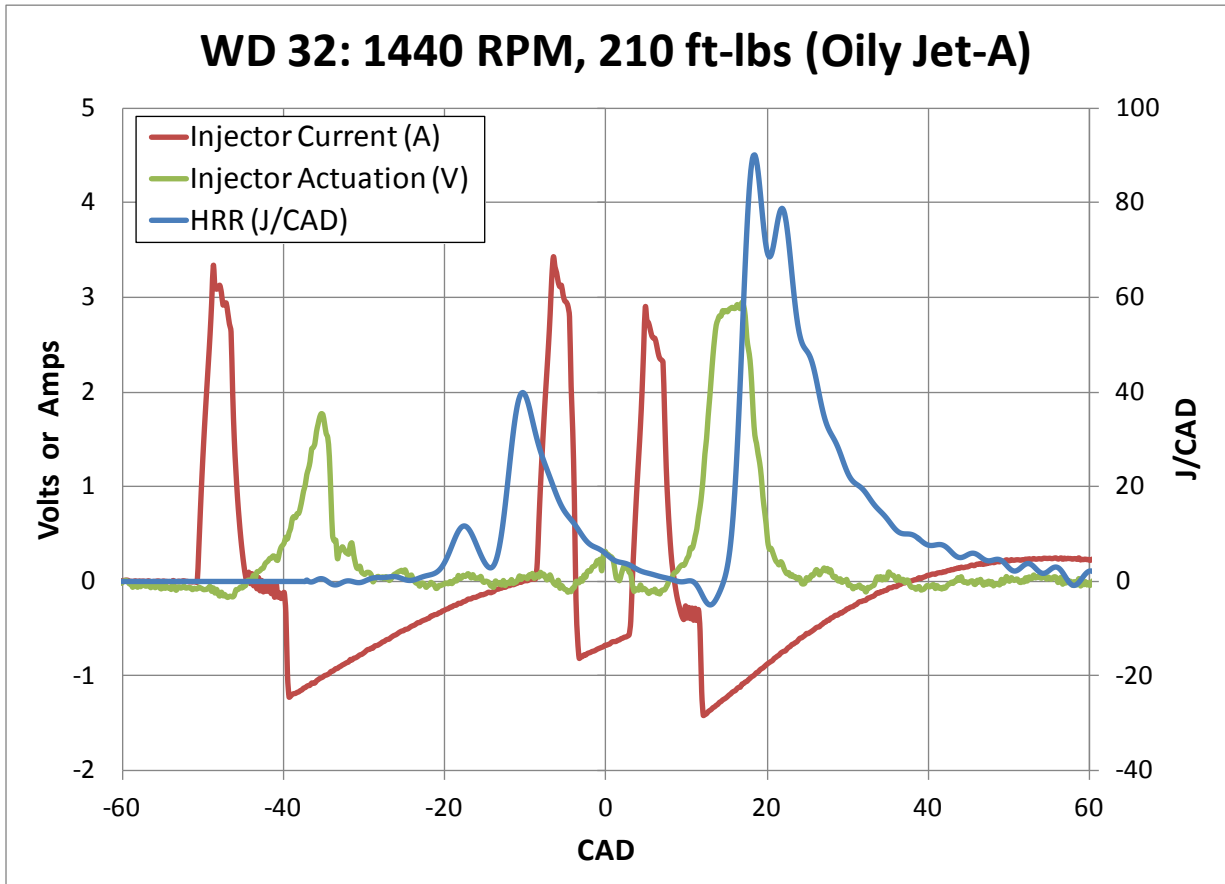
Figure 10. CAT C7 Comparison of Needle Lift and Coil Current with HRR Overlay
