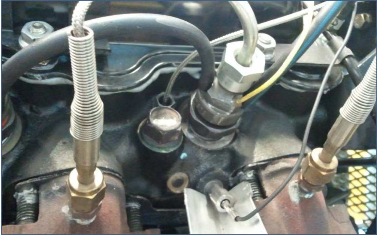
Figure 5. GE 6.5T Cylinder Pressure Transducers and Instrumented Injector
