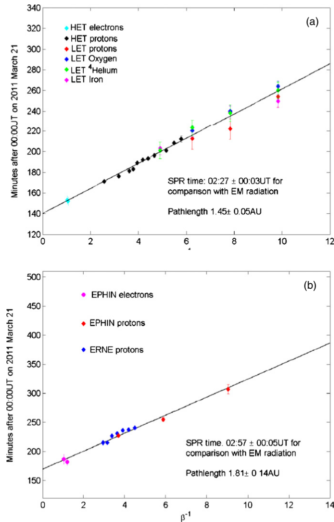
Figure 11. Top panel: a velocity dispersion analysis based on the measurements of the onset of electrons, light (protons), and heavy ions (oxygen, ^4\text{He} , and iron) at STA . Bottom panel: a velocity dispersion analysis based on the measurements of the onset of electrons and protons by EPHIN and the onset of protons by ERNE.
