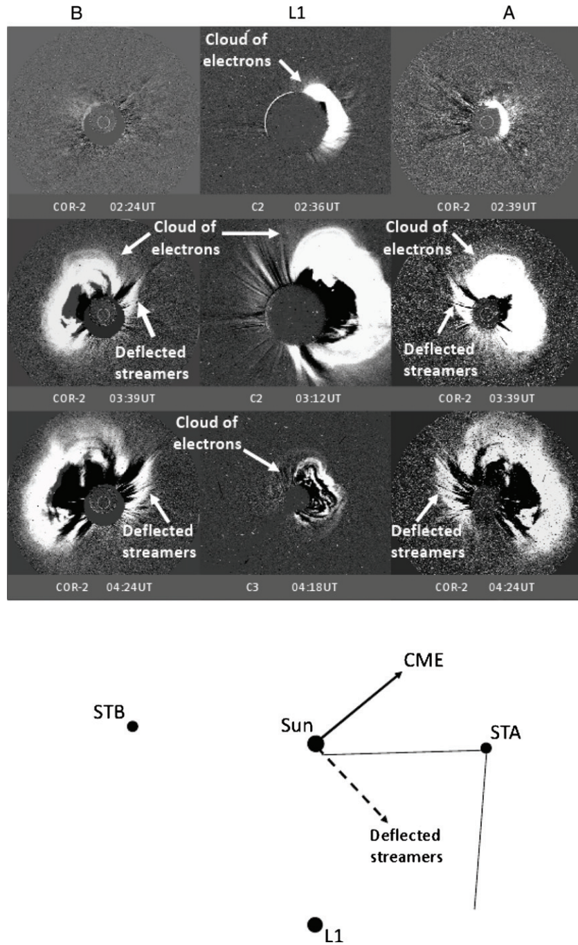
Figure 1. Running-difference images of the 2011 March 21 CME obtained by COR-2B (left-hand column), C2/C3 (middle column), and COR-2A (right-hand column). The “cloud of electrons” and deflected streamers are labeled.
