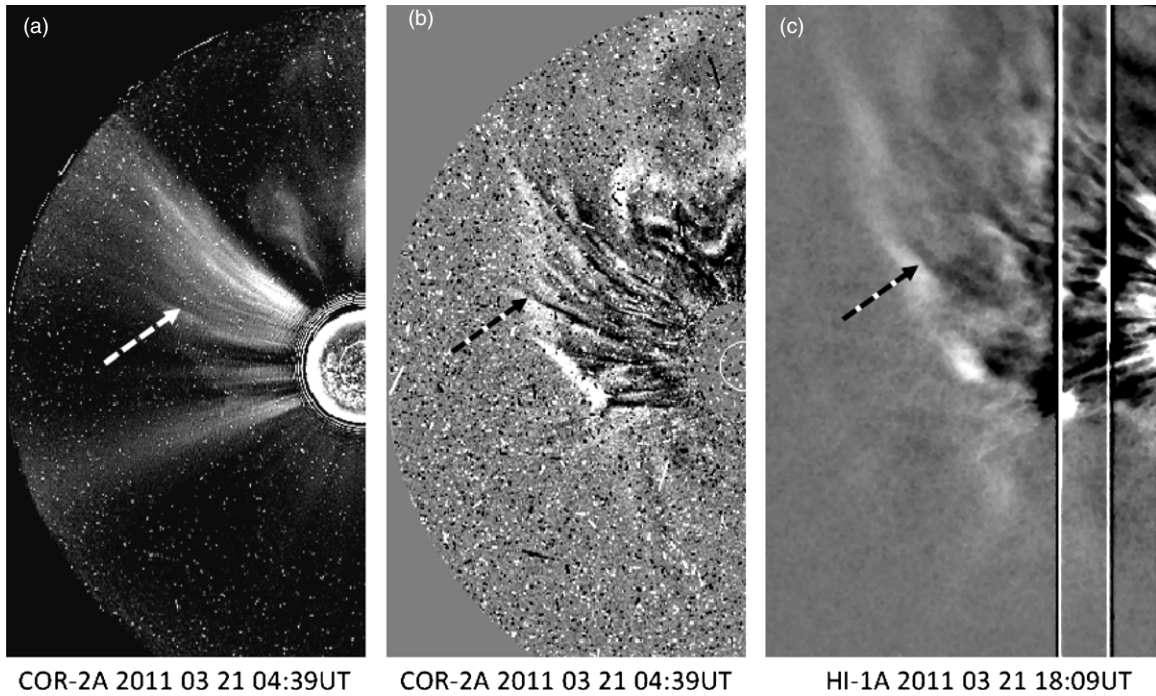
Figure 7. Left: a background-subtracted COR-2A image taken of the east limb of the Sun. Middle: the corresponding running-difference image; right: an HI-1A image of the deflected streamer stalk convected out with the compression wave of the CME. Arrows point to single streamer stalk convected out with the compression wave of the CME.
