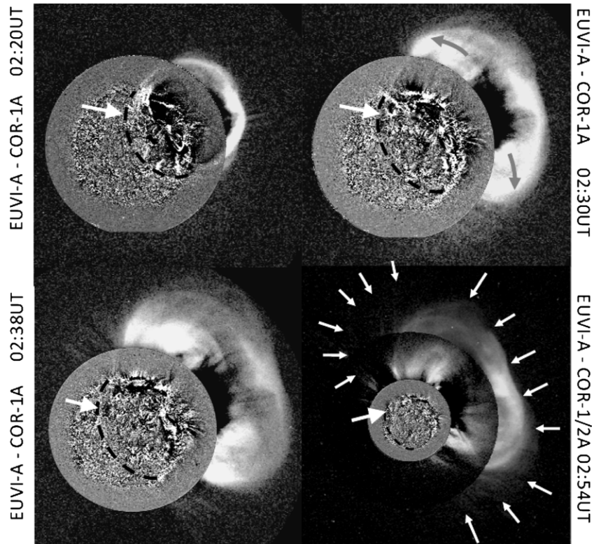
Figure 4. Combined COR-1A and EUVI-A images showing the relation between the propagating EUV disturbance tracked in the lower corona in 195 Å and the CME expanding in the upper corona in the COR-1A field of view at 02:20, 02:30, and 02:38 UT. Black dashed lines and thick white arrows mark the extent of the EUV wave. Bottom right-hand panel: combined EUVI-A, COR-1A, and COR-2A images at 02:54 UT. The thin white arrows shown in the COR-1/2A field of view mark the larger extent of the cloud of electrons surrounding the CME. The limits of this cloud were determined from the sharp drop in coronal brightness observed on its surface in the corresponding running-difference image (bottom left-hand panel of Figure 2).
