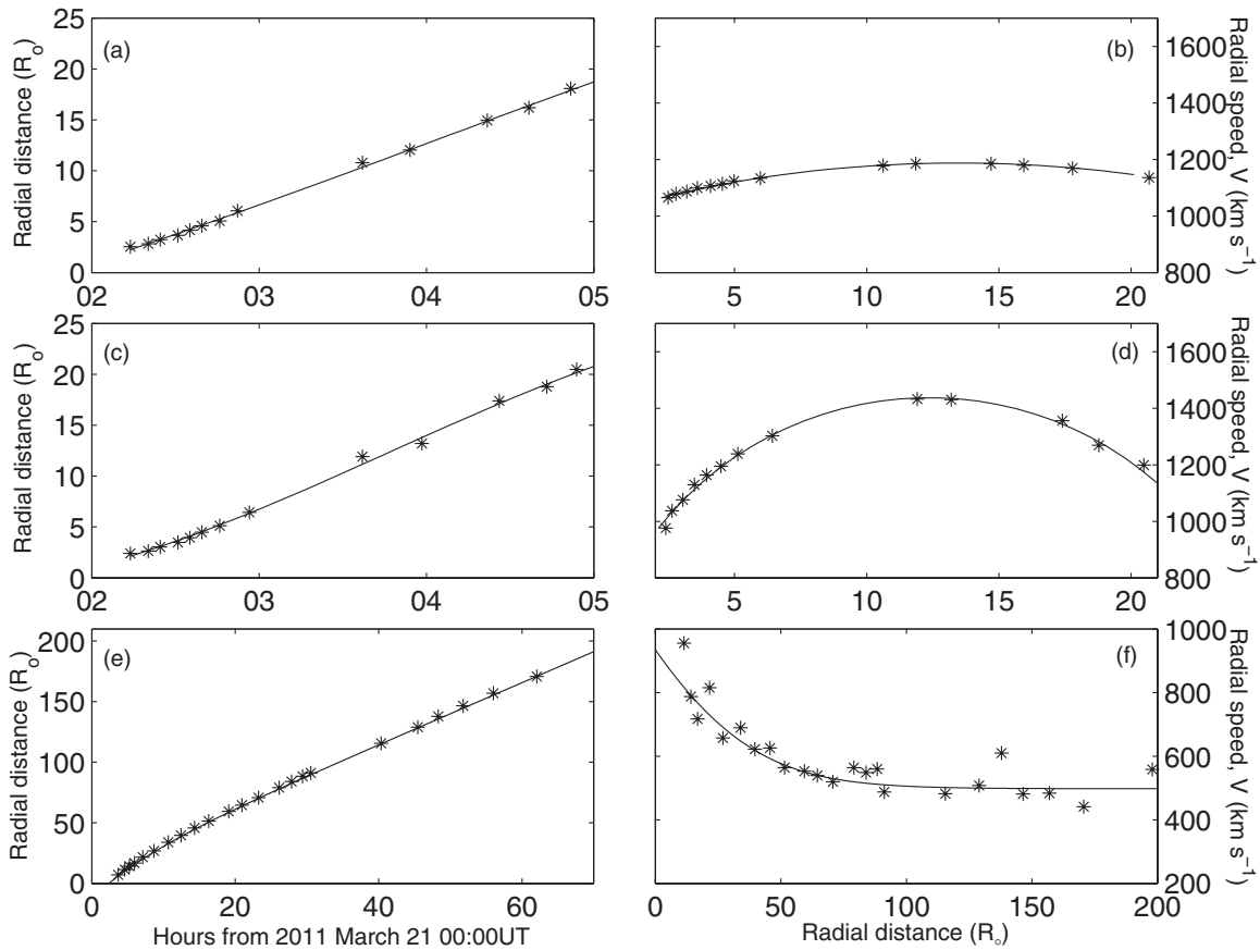
Figure 6. Three kinematic analysis made at different position angles (top: 296°, middle: 275°, bottom: 91° as shown in Figure 2). The radial distance of the leading edge of the cloud of electrons measured along these three position angles is shown in the left-hand panel, the derived radial component of the shock speed is shown in the right-hand panel. The measurements made along lines of constant position angles located in the ecliptic plane and connected to the STA and L1 particle detectors are shown in the middle and bottom panels, respectively. The functional forms that model the speed variations best are third-order polynomial fits (top and middle panels) and a decaying exponential for the bottom panel. Note that the CME-driven compression region is tracked over much longer radial distances in the bottom panels since the HI-1/2A running-difference images can be used.
