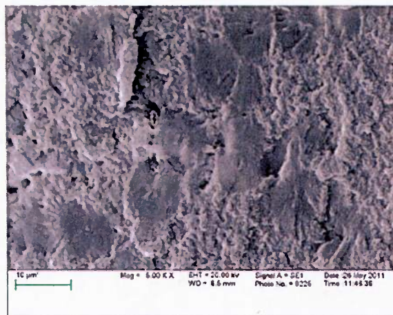
Figure 19. SEM photo of surface morphology of a sample with IPTES and TMSPM after brittle failure.
