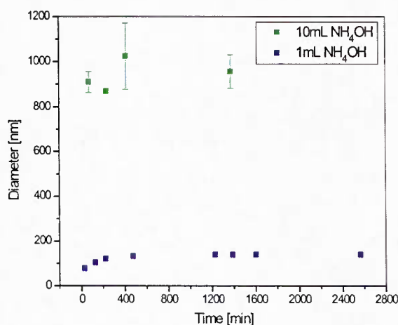
Figure 16. Light scattering results showing different diameters created by varying the ratio of ammonium hydroxide to water.
