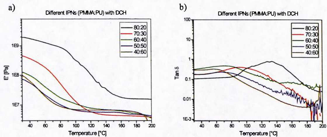
Figure 4. E' and T_g values of IPNs with DCH, an inhibitor present in the PMMA phase, and with different ratios of PMMA:PU
