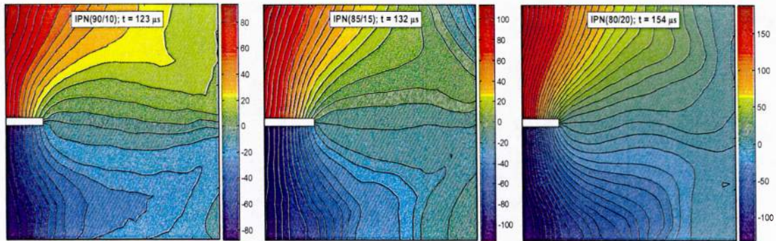
Figure 7 – Crack-opening ( v -field) displacement contours for different IPNs. (Contour interval: 7 \mu\text{m} .) Color-bars indicate displacements in \mu\text{m} .
