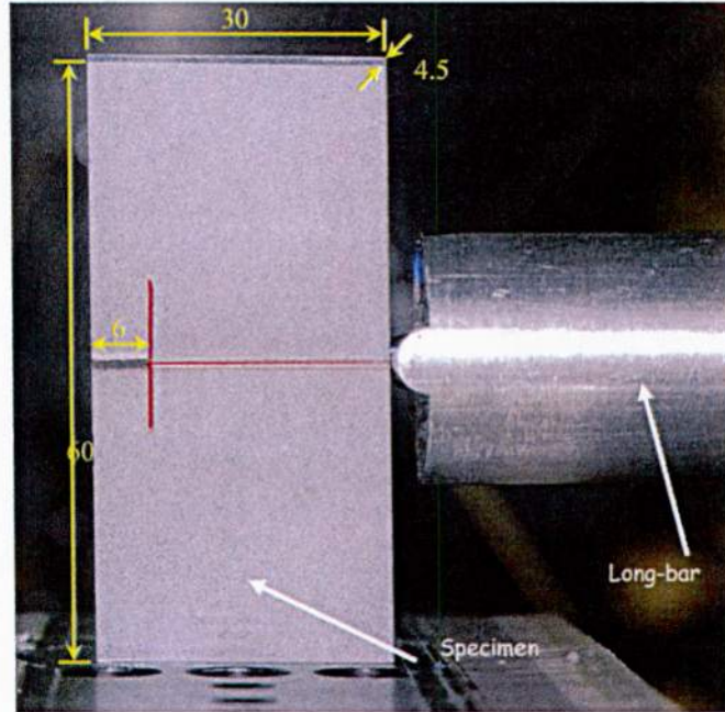
Figure 5 – Close-up view of mode-I specimen geometry used for fracture testing of t -IPNs. Dimensions in mm. (color photo)
