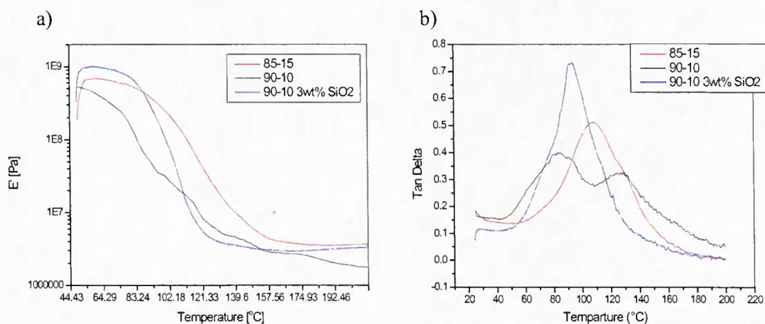
Figure 18. DMA results showing the Young's modulus (a) and T_g (b) of the IPN systems with the silica particles included.
