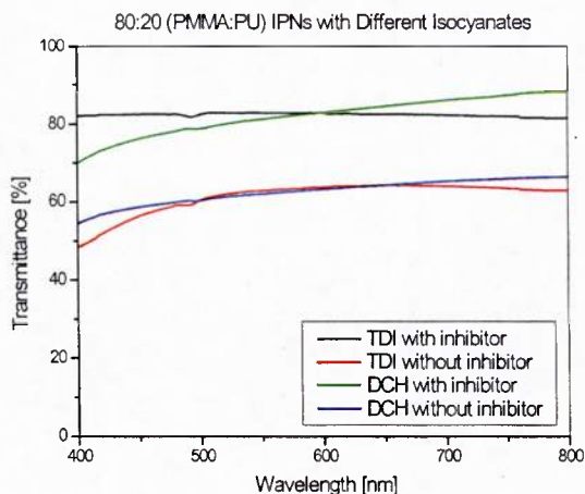
Figure 2. UV-visible results showing IPNs consisting of 80 wt% PMMA and 20 wt% PU with different isocyanates
