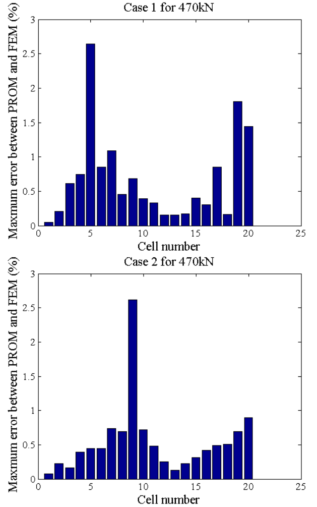
Figure 12. Maximum errors between PROM and FEM for each cell (center node displacement) in the frequency range of interest for cases 1 (top) and 2 (bottom) with 470kN pre-stress
