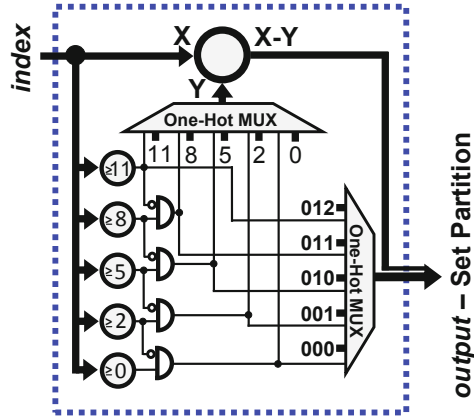
Fig. 3. Single-Stage Index to Set Partition Circuit for n = 4
