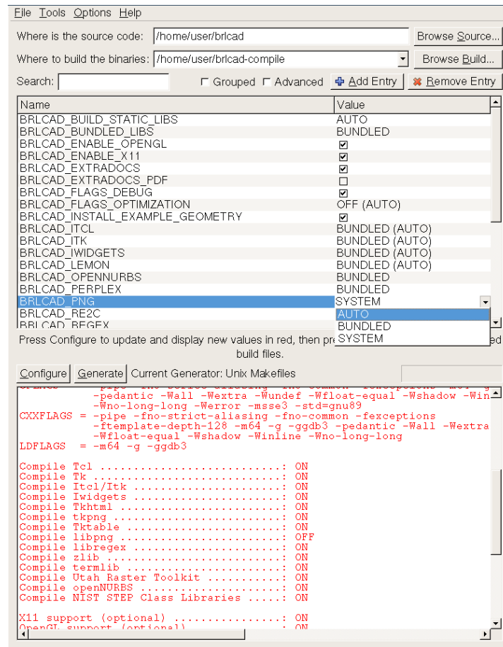
Figure 14. CMake GUI drop-down menu options.
