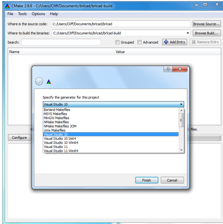
Figure 4. cmake-gui showing MSVC generator options.
