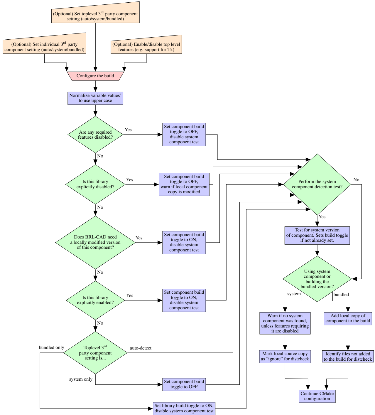
Figure 13. Logical flow of third party component configuration.
