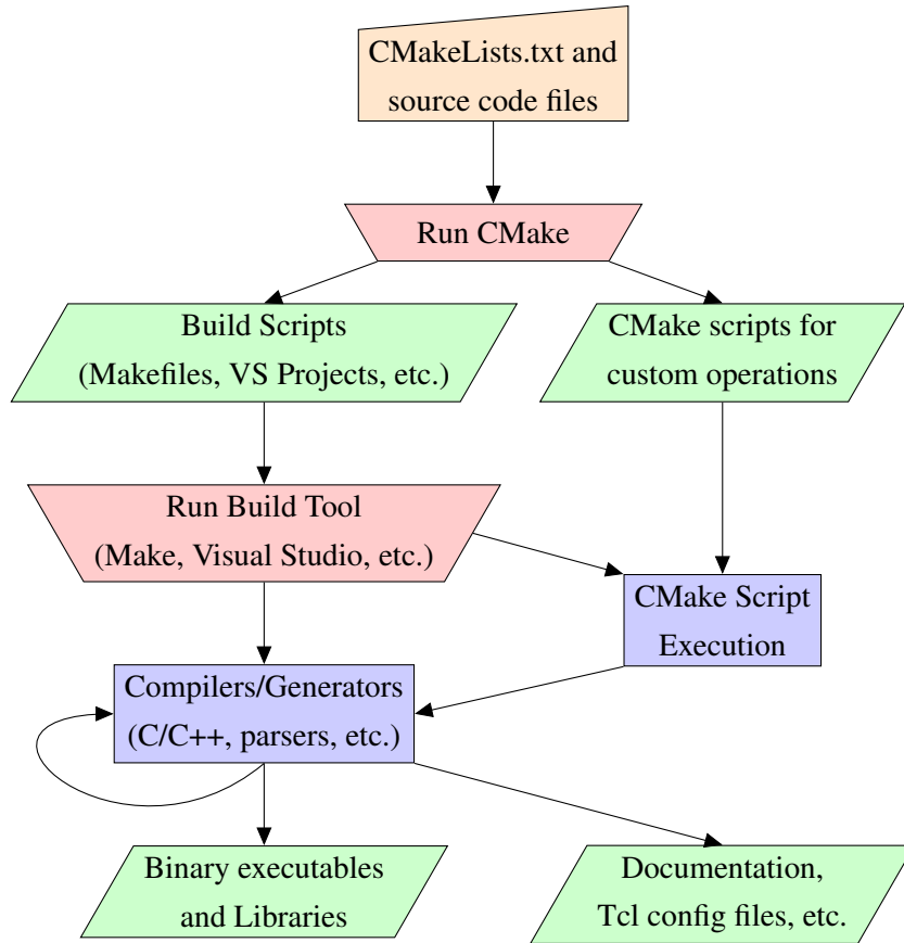
Figure 1. High level flowchart of BRL-CAD's build process.
