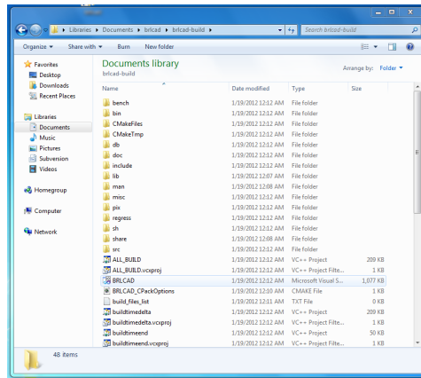
Figure 7. MSVC project generated by CMake.
