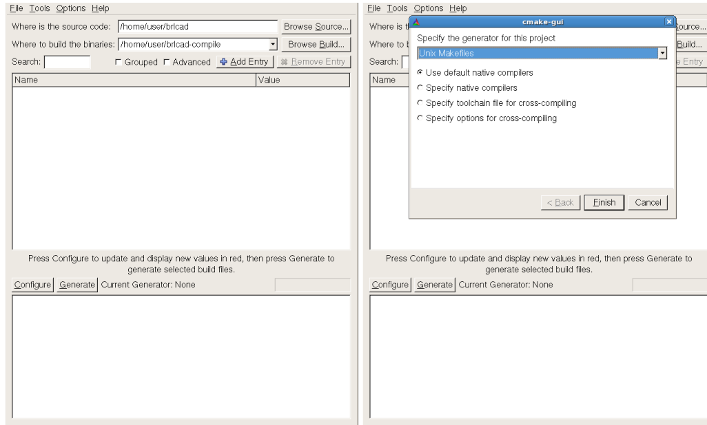
Figure 2. (left) Initial cmake-gui screen and (right) dialog allowing the user to select the build tool for which inputs will be generated.
