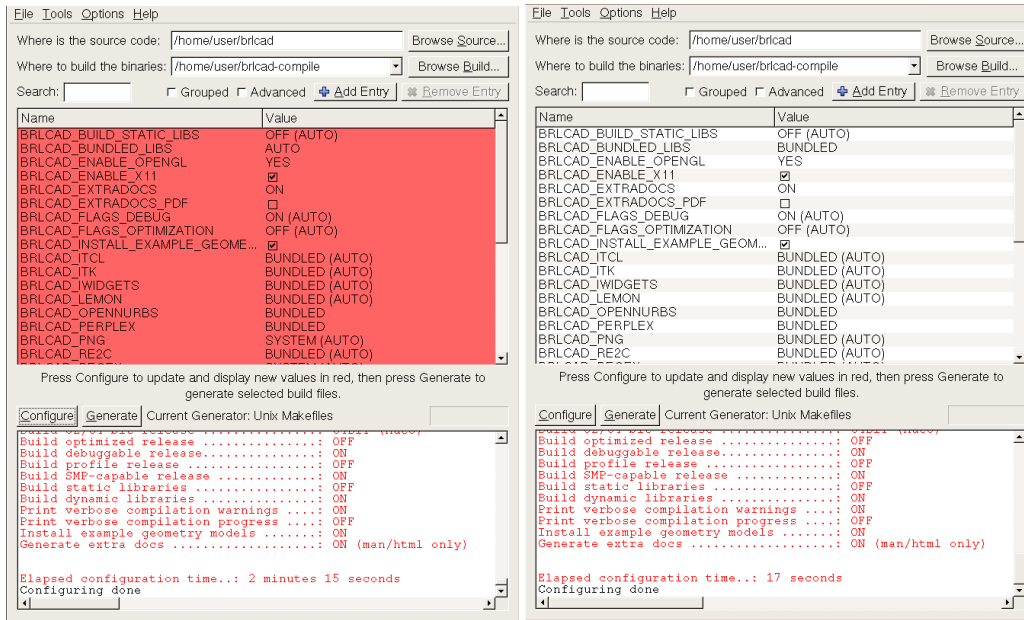
Figure 3. The CMake variable list after the first configure pass (left) and second configure pass (right). After two passes, no new variables are present — ready to generate.
