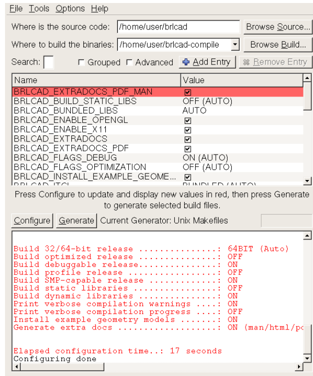
Figure 16. Addition of PDF variable after enabling PDF output.
