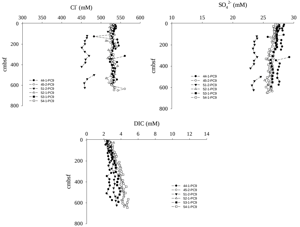
Figure 12: Pore water \text{SO}_4^{2-} , \text{Cl}^- and DIC profiles in cores from the eastern side of the pockmark at Site 1.
