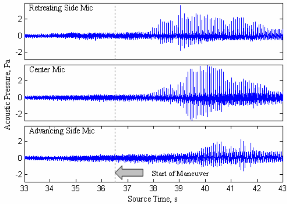
Figure 2.13. Acoustic time history during moderate pull-up maneuver.
