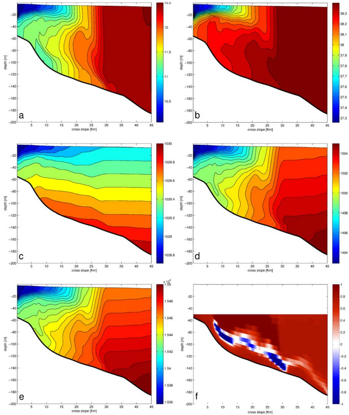
FIGURE 2. Model output of the grid line relative to S08 or AS07 seismic acquisition line. Upper panels: potential temperature(left) and salinity (right). Central panel: in situ density and sound speed. Lower panel: acoustic impedance and acoustic reflectivity.
